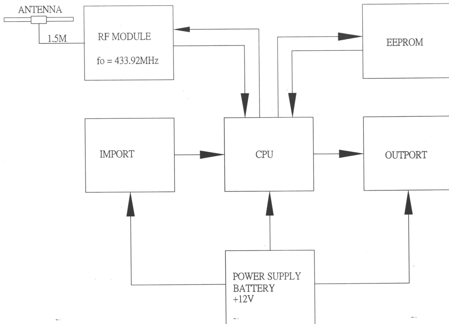
BLOCK DIAGRAM OF RECIVER-
