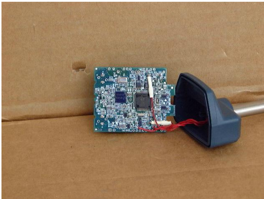
Figure 3 PCB 1 Side 2
