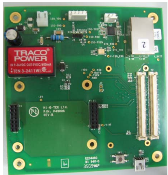
Main board #P49006 REV-B w/o modules
