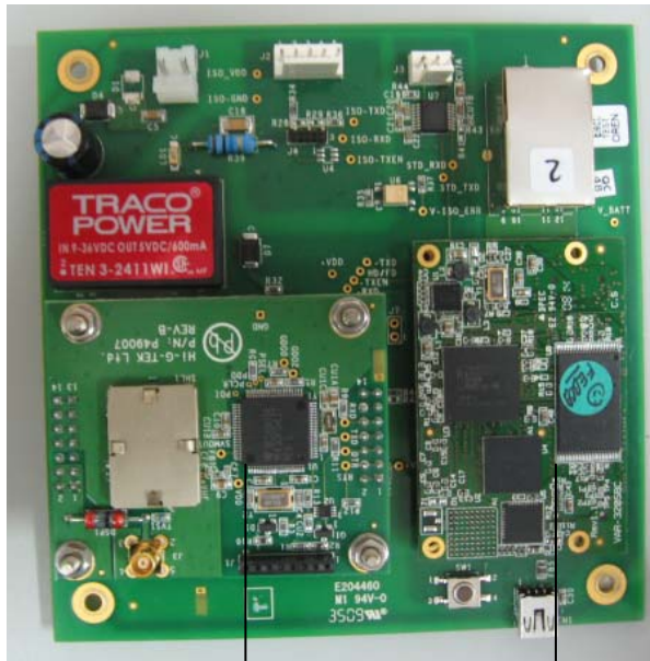
Main board #P49006 REV-B with modules
