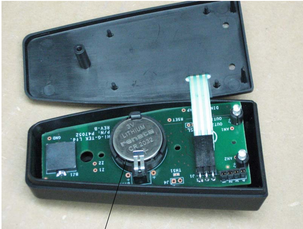
Internal Circuit board Top
