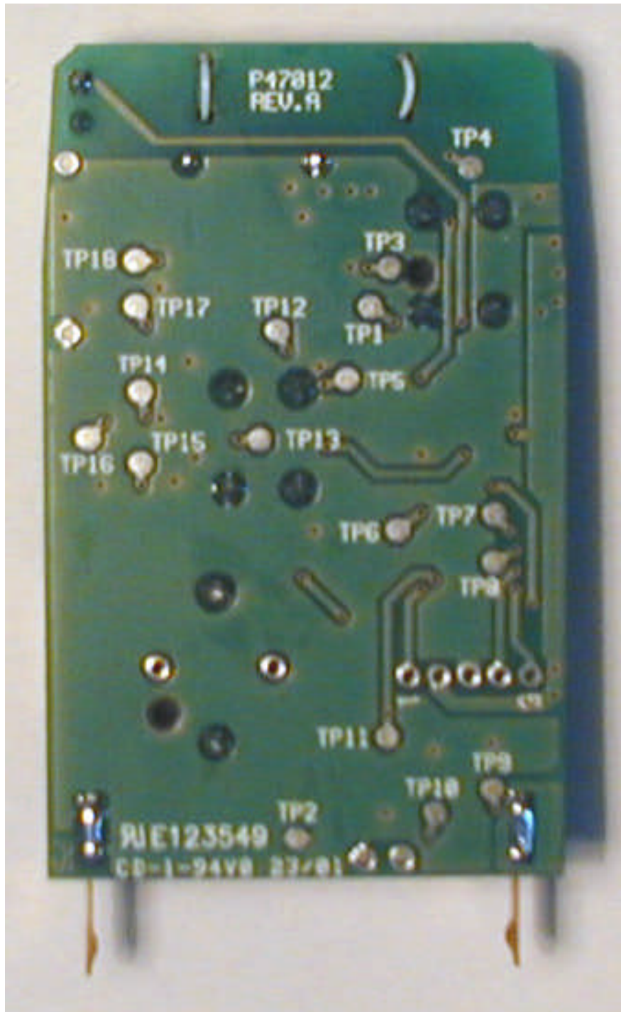
Photograph No.2 PCB printed side
