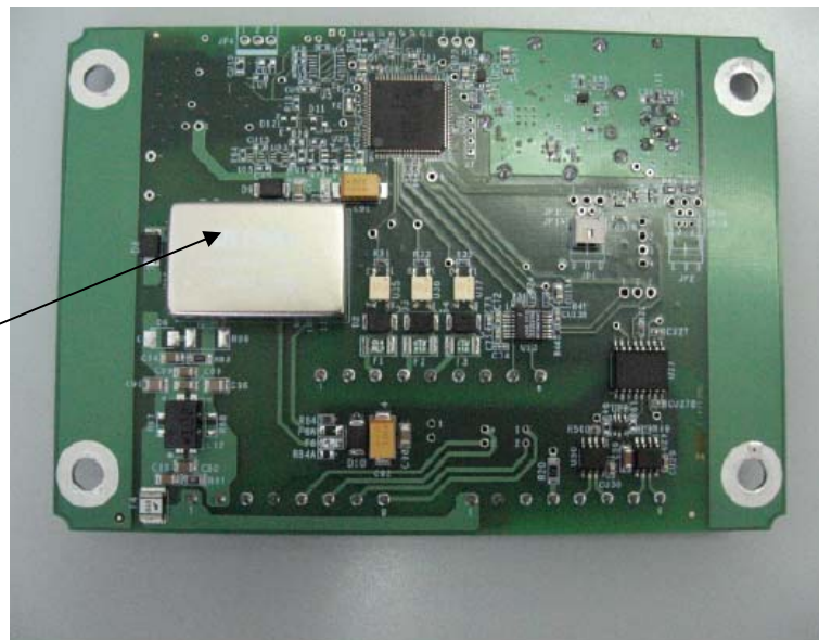
Figure 3 PCB Side 1 IG-CR-46D-916
