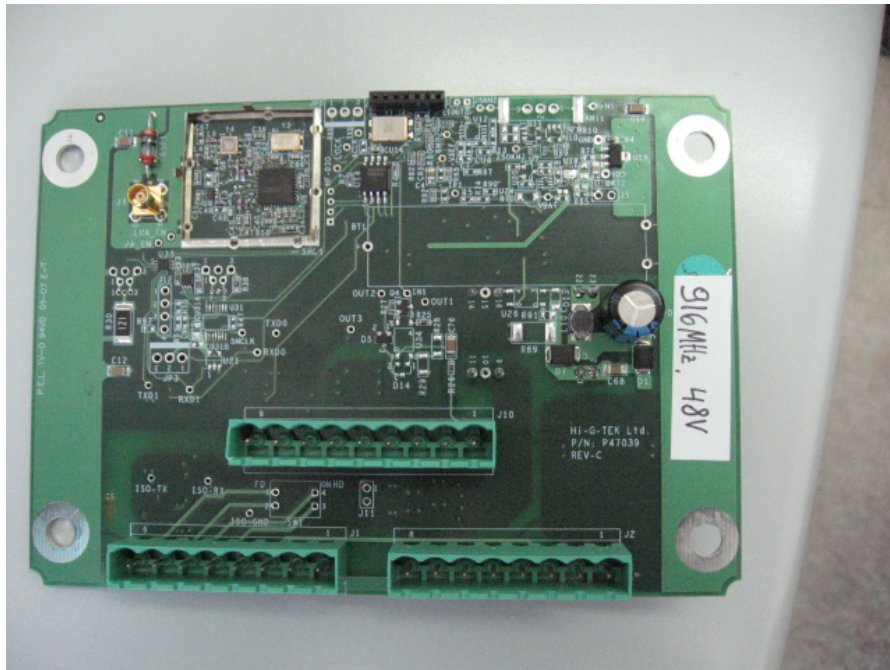
Figure 8 PCB Side 2 IG-CR-86D-916
