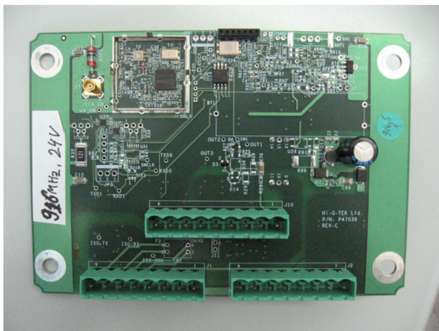
Figure 4 PCB Side 2 IG-CR-46D-916
