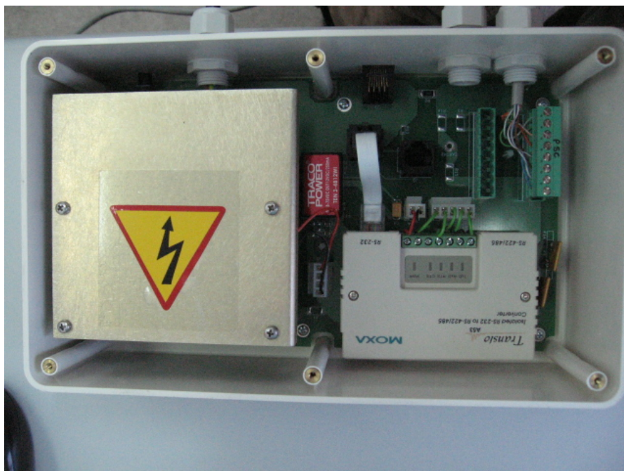
Figure Internal View PS IG-PS-4RI/ IG-PS-8RI
