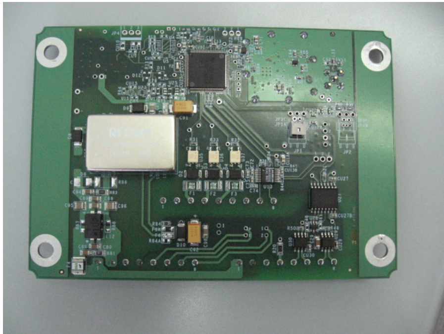
Figure 3 PCB Side 1 IG-CR-46D-916
