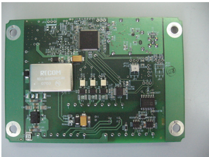
Figure 7 PCB Side 1 IG-CR-86D-916
