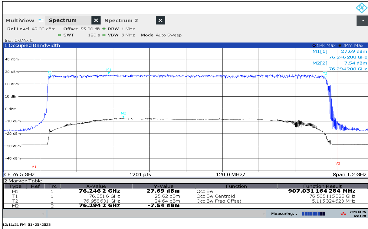
Plot 14: OBW, Mode 27, T_{min} / V_{min-max}
