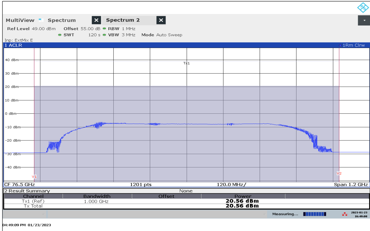
Plot 49: EIRP Mean Power (Channel Power), Mode 63, RMS detector, T_{nom} / V_{min-max}
