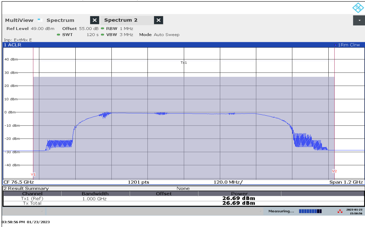
Plot 34: EIRP Mean Power (Channel Power), Mode 15, RMS detector, T_{nom} / V_{min-max}
