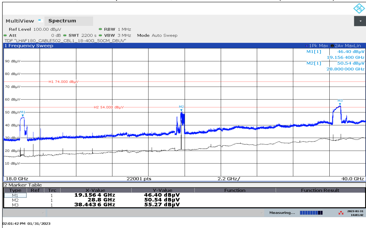
Plot 58: 18 GHz – 40 GHz, valid for specified modes, antenna vertical / horizontal (PEAK detector)
