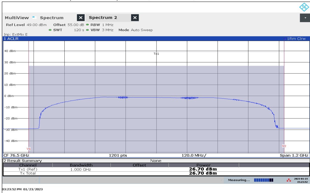
Plot 28: EIRP Mean Power (Channel Power), Mode 03, RMS detector, T_{nom} / V_{min-max}
