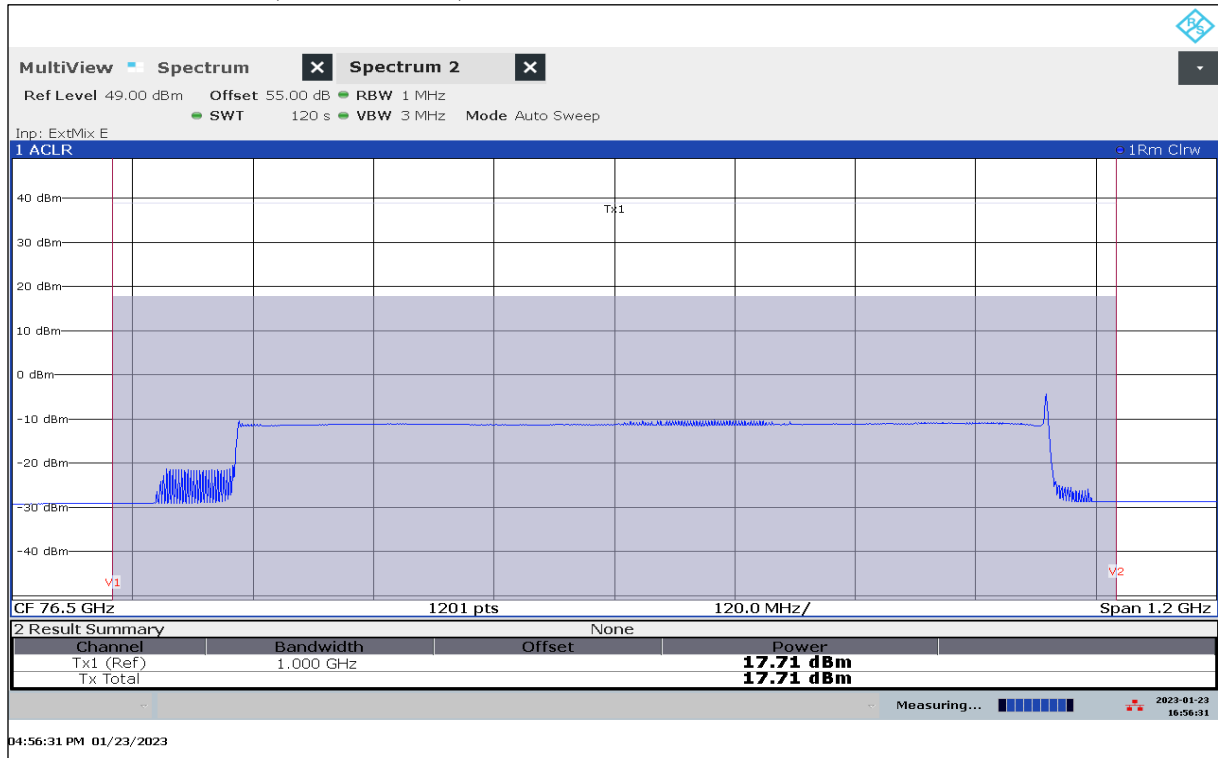
Plot 52: EIRP Mean Power (Channel Power), Mode 80, RMS detector, T_{nom} / V_{min-max}
