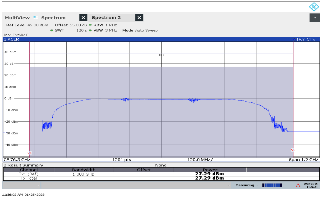
Plot 38: EIRP Mean Power (Channel Power), Mode 21, RMS detector, T_{min} / V_{min-max}
