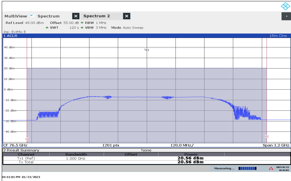
Plot 46: EIRP Mean Power (Channel Power), Mode 51, RMS detector, T_{nom} / V_{min-max}
