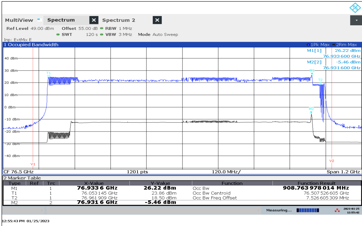
Plot 26: OBW, Mode 80, T_{min} / V_{min-max}
