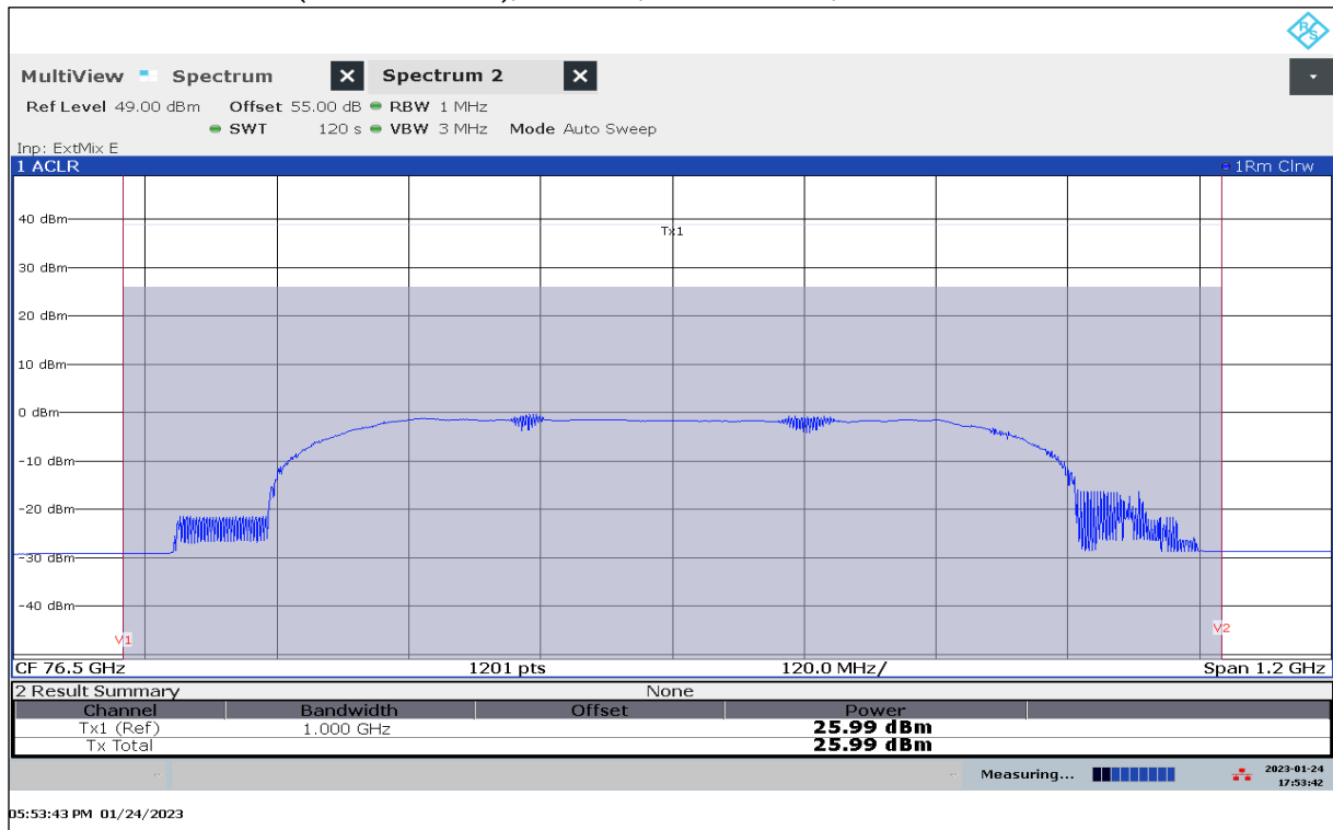
Plot 36: EIRP Mean Power (Channel Power), Mode 15, RMS detector, T_{max} / V_{min-max}
