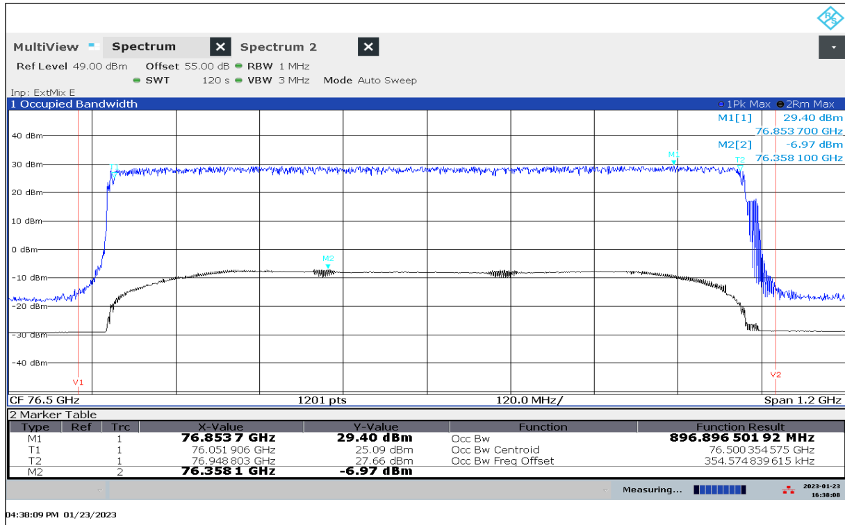
Plot 16: OBW, Mode 39, T_{nom} / V_{min-max}
