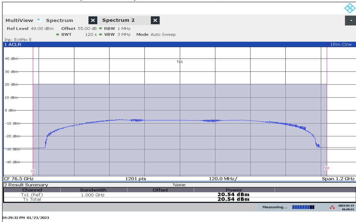
Plot 40: EIRP Mean Power (Channel Power), Mode 27, RMS detector, T_{nom} / V_{min-max}
