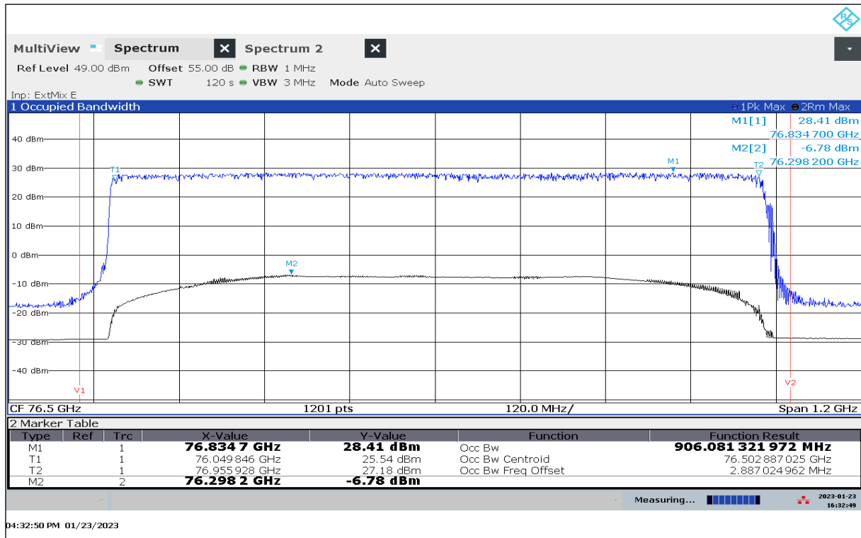
Plot 13: OBW, Mode 27, T_{nom} / V_{min-max}
