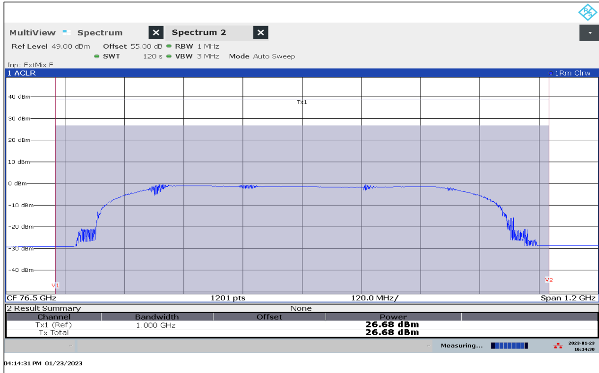
Plot 37: EIRP Mean Power (Channel Power), Mode 21, RMS detector, T_{nom} / V_{min-max}
