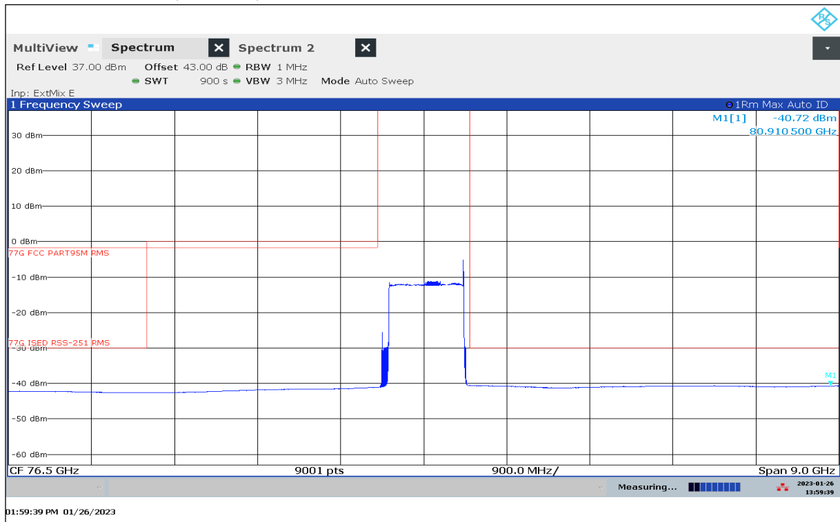
Plot 72: 72 GHz – 81 GHz, Mode 80, antenna vertical / horizontal
