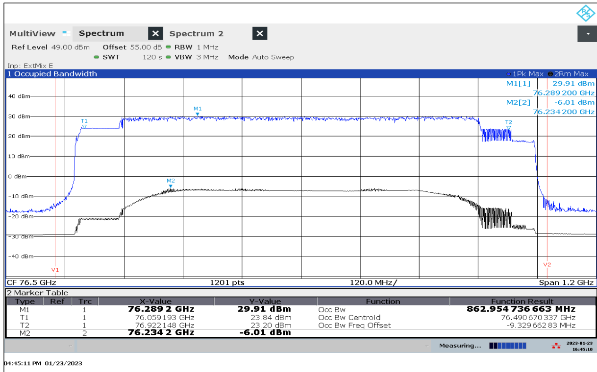
Plot 19: OBW, Mode 51, T_{nom} / V_{min-max}
