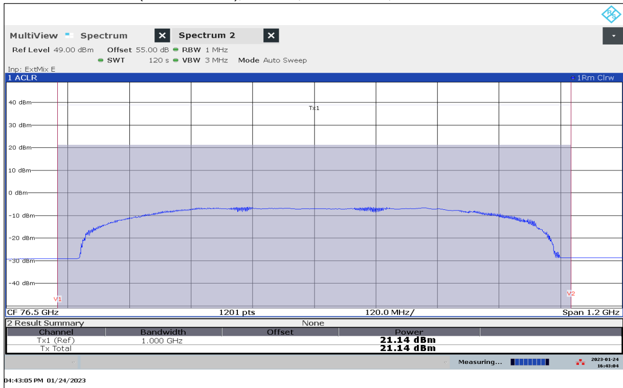
Plot 42: EIRP Mean Power (Channel Power), Mode 27, RMS detector, T_{max} / V_{min-max}
