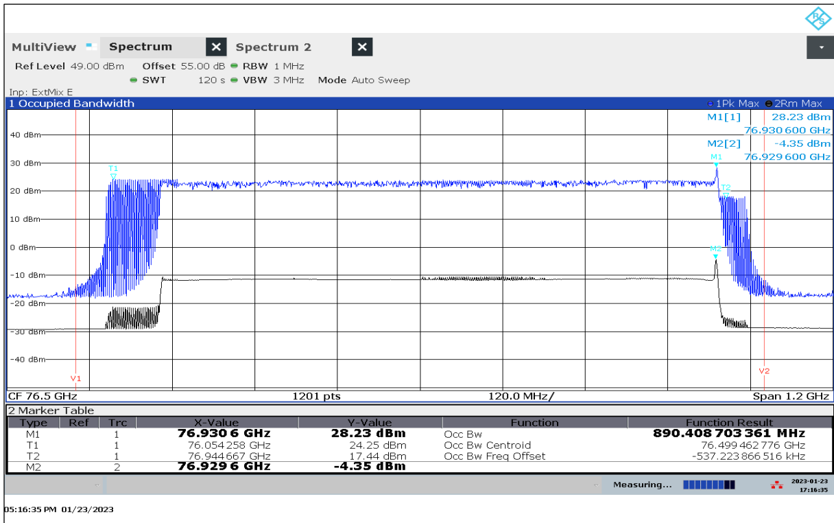
Plot 25: OBW, Mode 80, T_{nom} / V_{min-max}
