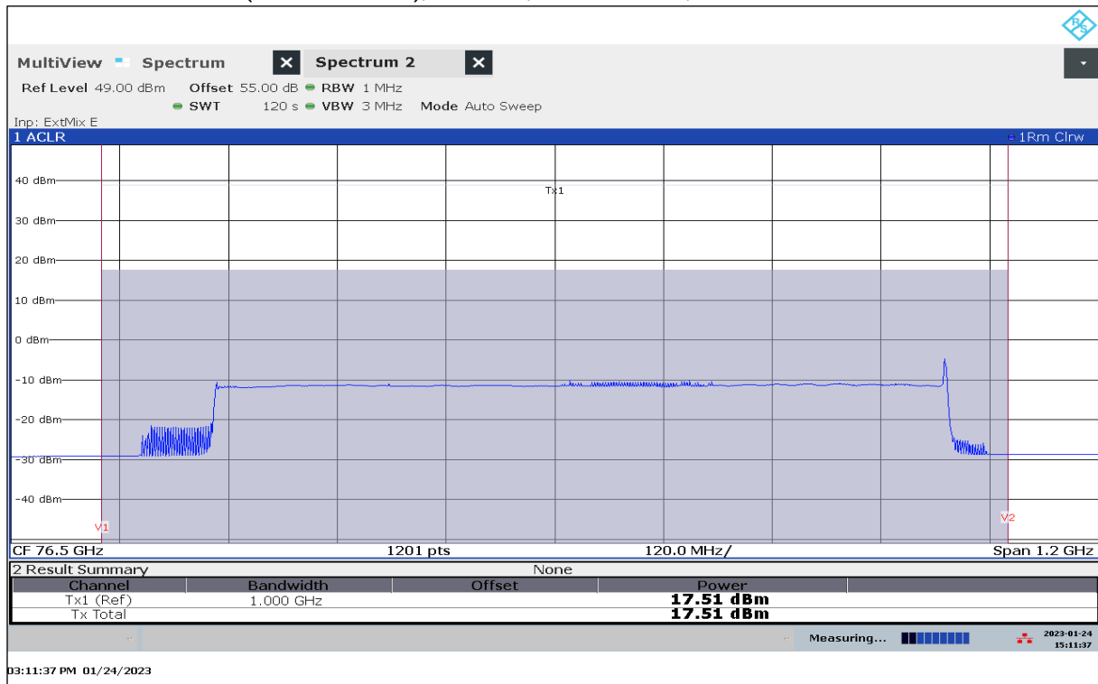
Plot 54: EIRP Mean Power (Channel Power), Mode 80, RMS detector, T_{max} / V_{min-max}
