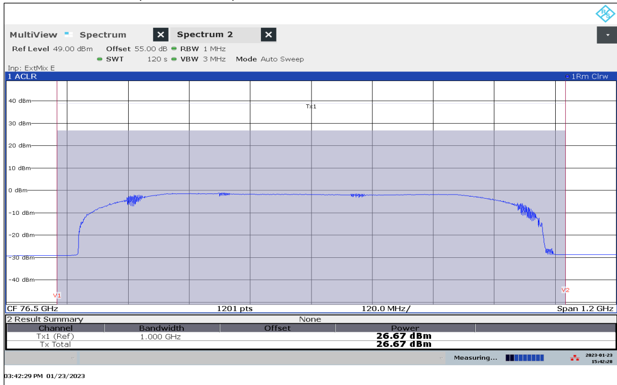
Plot 31: EIRP Mean Power (Channel Power), Mode 09, RMS detector, T_{nom} / V_{min-max}
