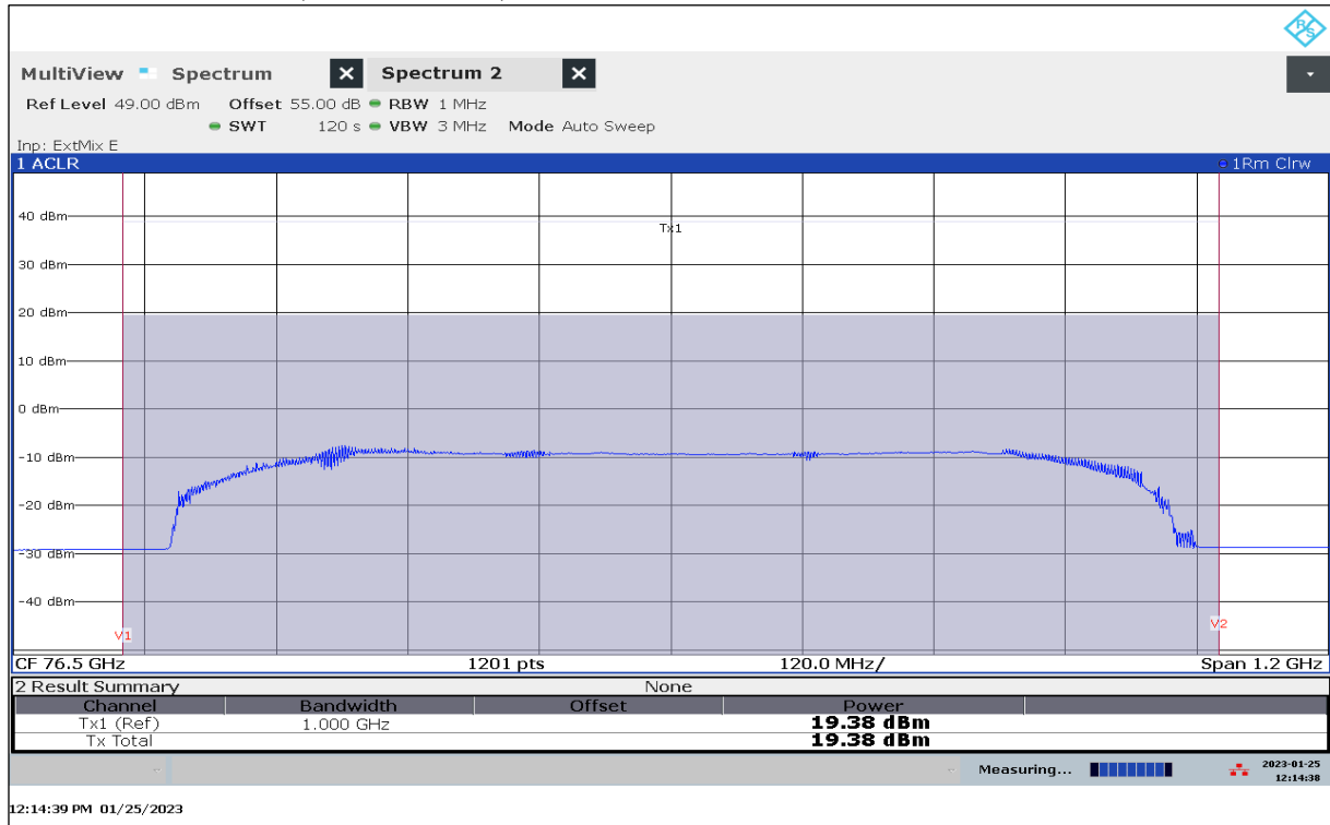
Plot 44: EIRP Mean Power (Channel Power), Mode 39, RMS detector, T_{min} / V_{min-max}
