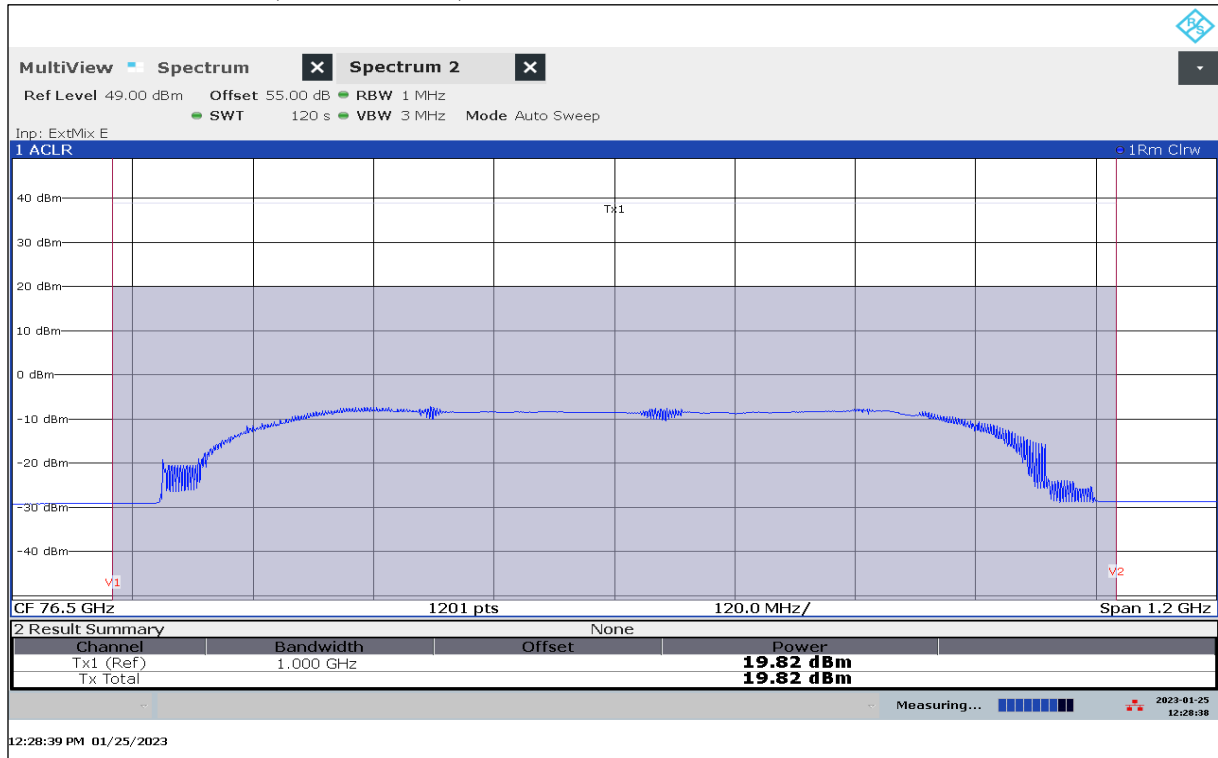
Plot 50: EIRP Mean Power (Channel Power), Mode 63, RMS detector, T_{min} / V_{min-max}
