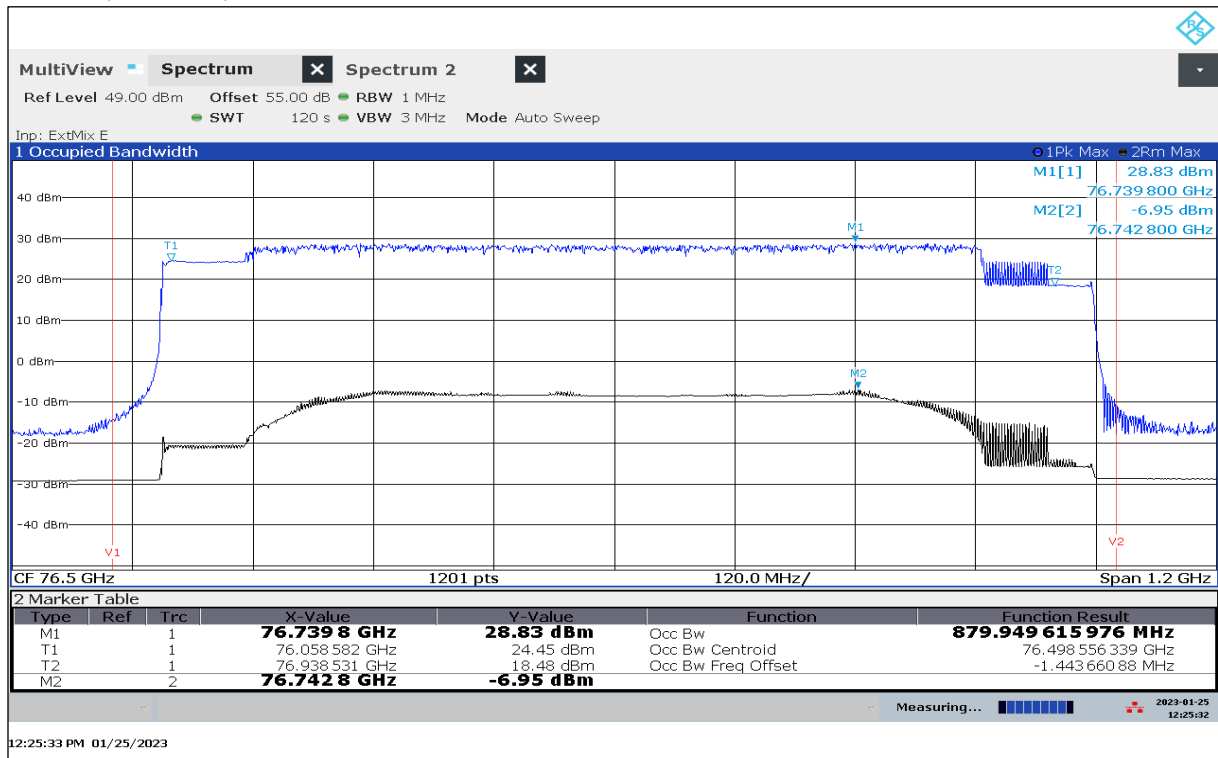
Plot 20: OBW, Mode 51, T_{min} / V_{min-max}
