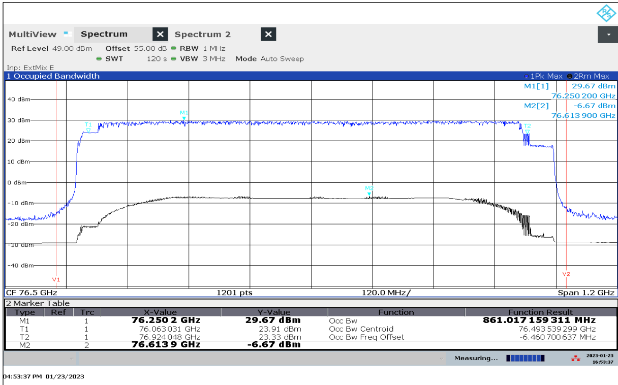
Plot 22: OBW, Mode 63, T_{nom} / V_{min-max}
