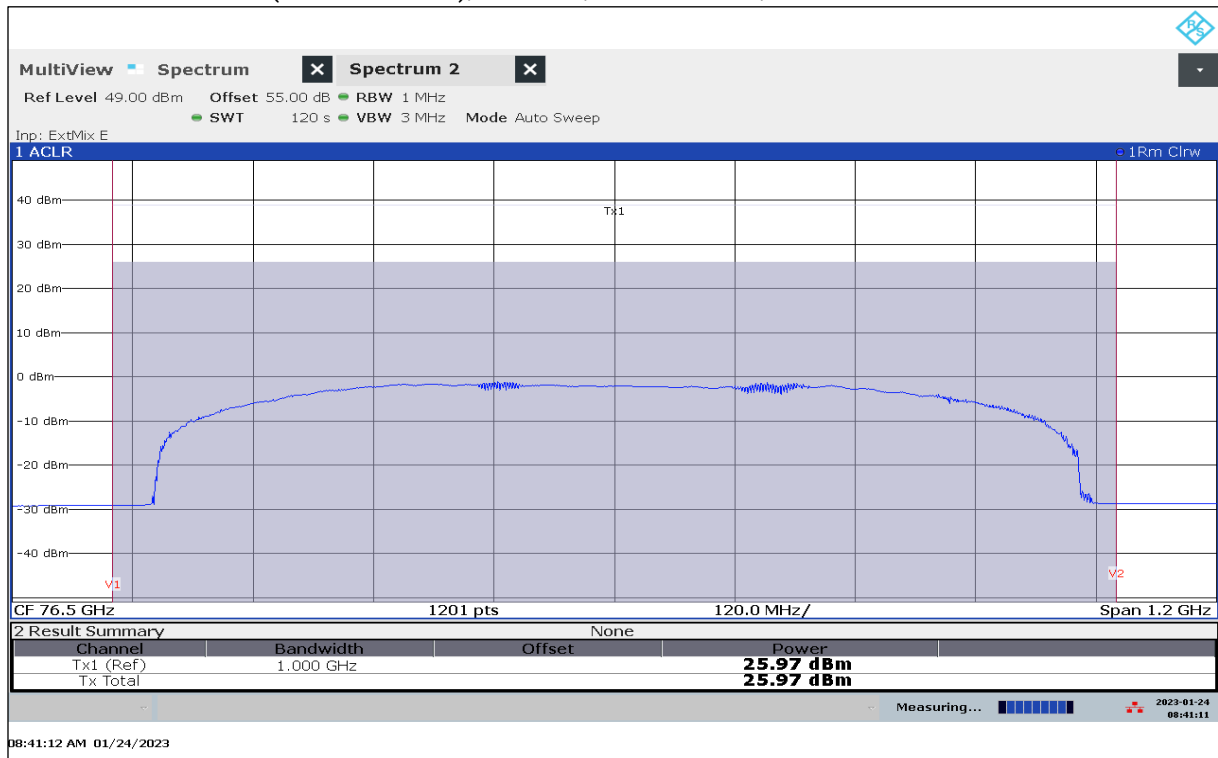
Plot 30: EIRP Mean Power (Channel Power), Mode 03, RMS detector, T_{max} / V_{min-max}
