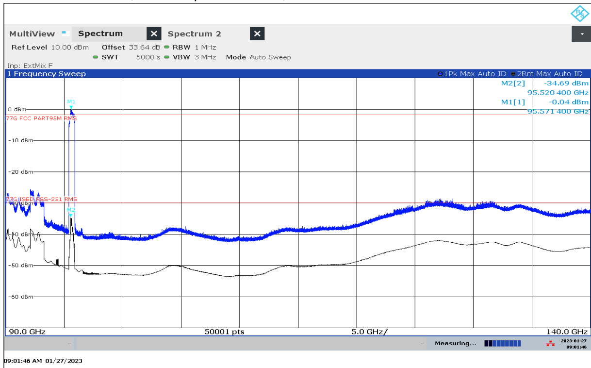
Plot 74: 90 GHz – 140 GHz, valid for specified modes, antenna vertical / horizontal
