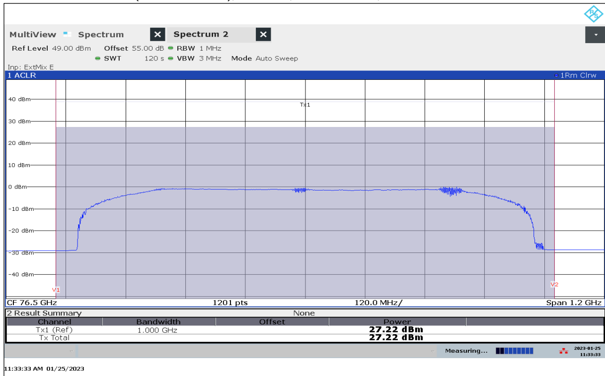
Plot 32: EIRP Mean Power (Channel Power), Mode 09, RMS detector, T_{min} / V_{min-max}
