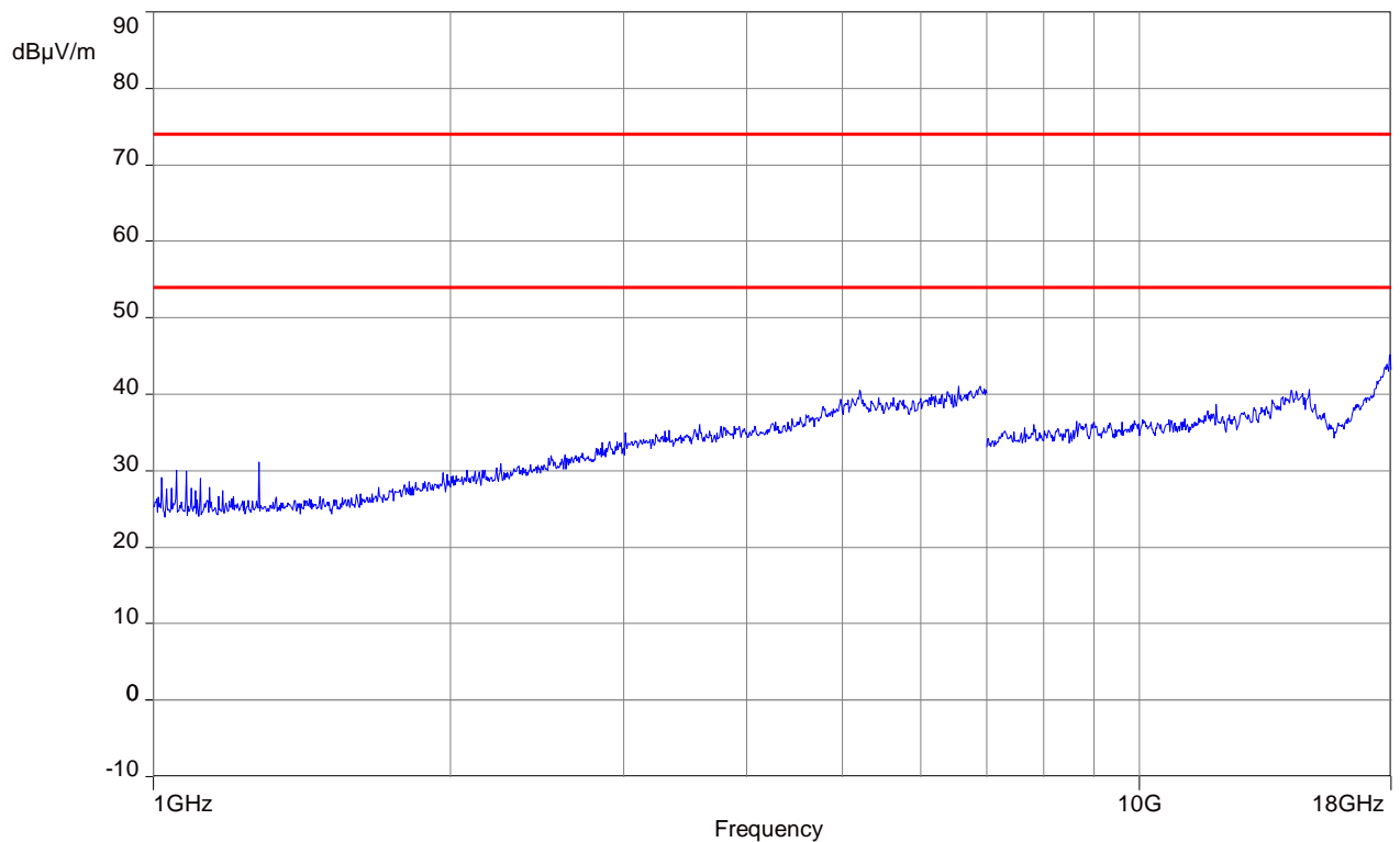
Plot 9: 1 GHz to 18 GHz, Mode 9(b)
