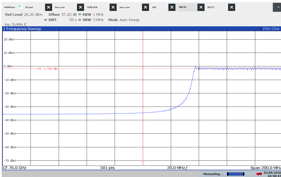
Plot 5: Mode 9(b), lower BEC
