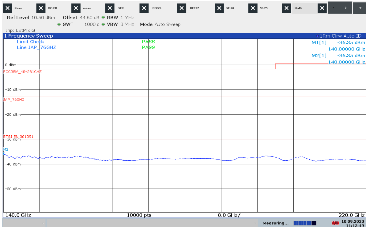
Plot 17: 140 GHz to 220 GHz, Mode 9(b)
