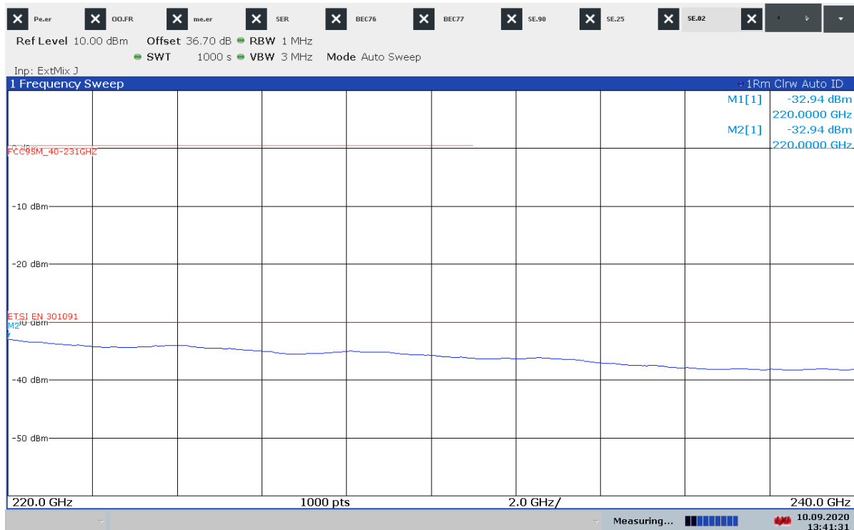
Plot 18: 220 GHz to 240 GHz, Mode 9(b)
