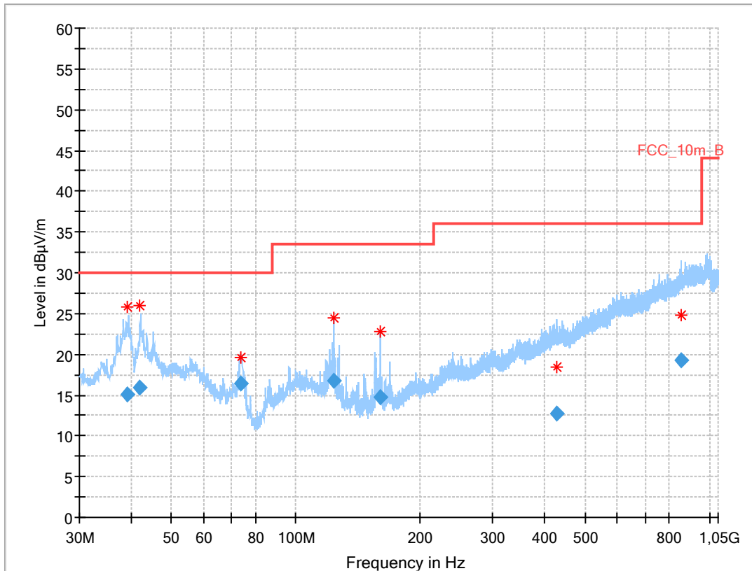
Plot 8: 30 MHz to 1 GHz, Mode 9(b)
