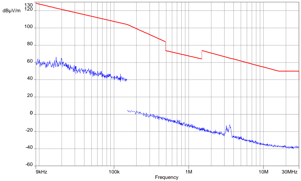
Plot 7: 9 kHz to 30 MHz, Mode 9(b)
