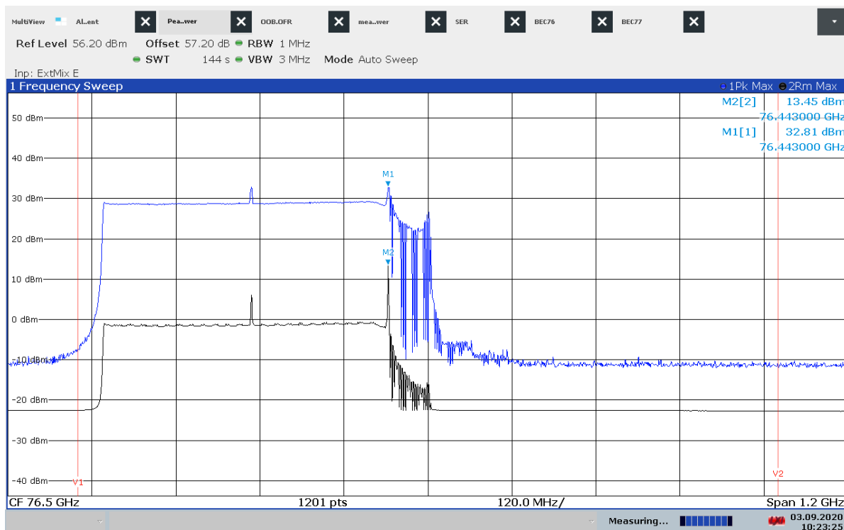
Plot 1: Mode 9(b), Radiated peak power, T_{nom} / V_{nom}
