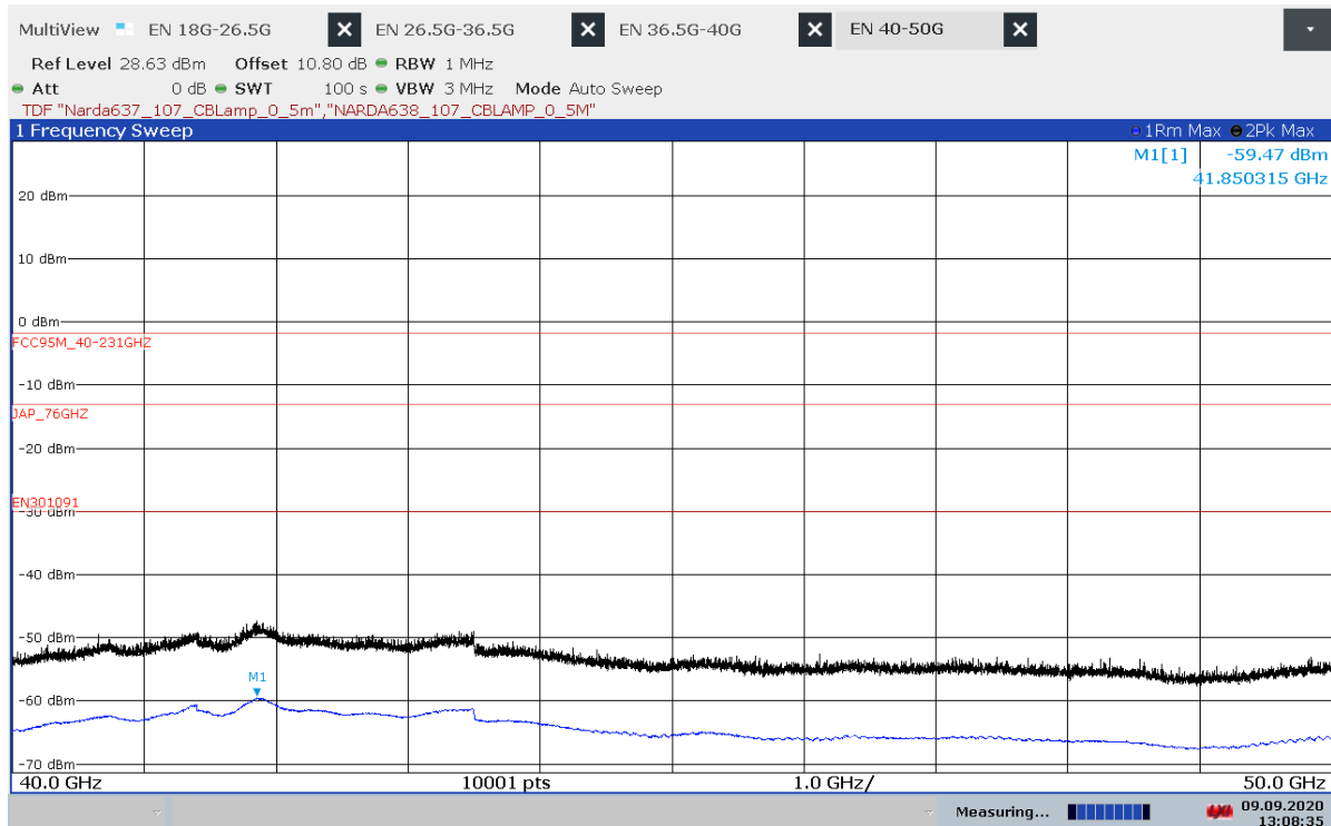
Plot 12: 40 GHz to 50 GHz, Mode 9(b)
