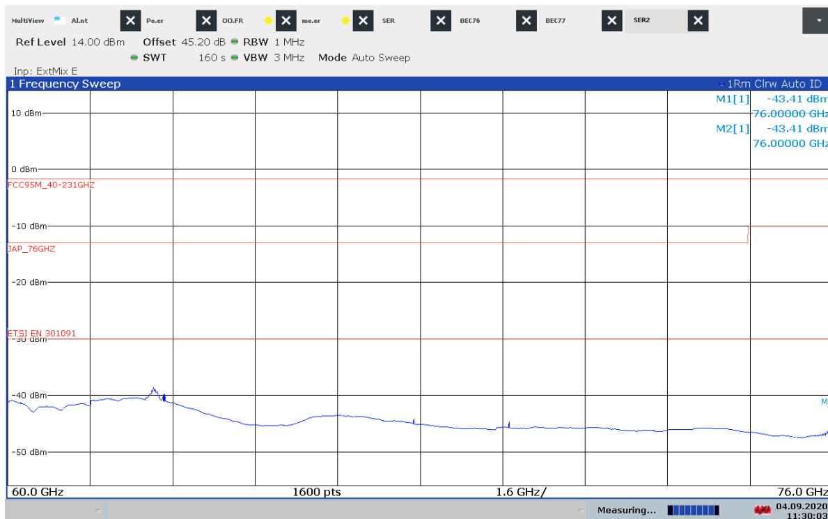
Plot 14: 60 GHz to 76 GHz, Mode 9(b)
