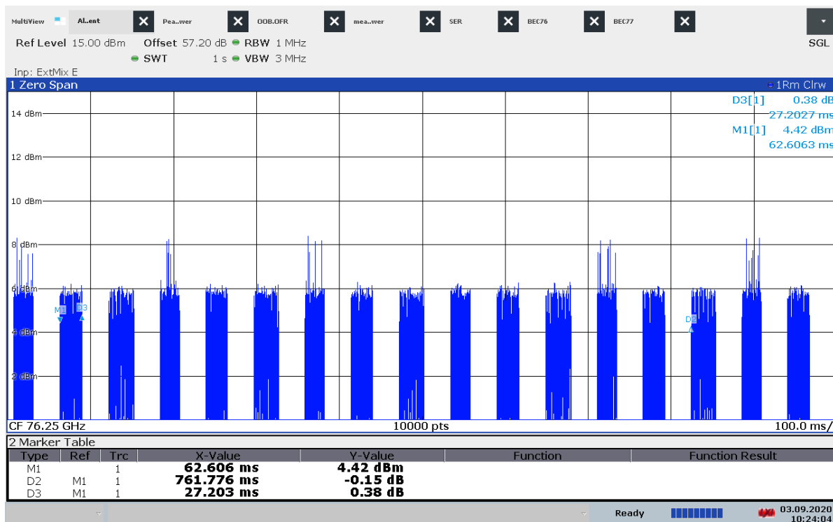
Plot 3: Mode 9(b), Time domain 76.25 GHz
