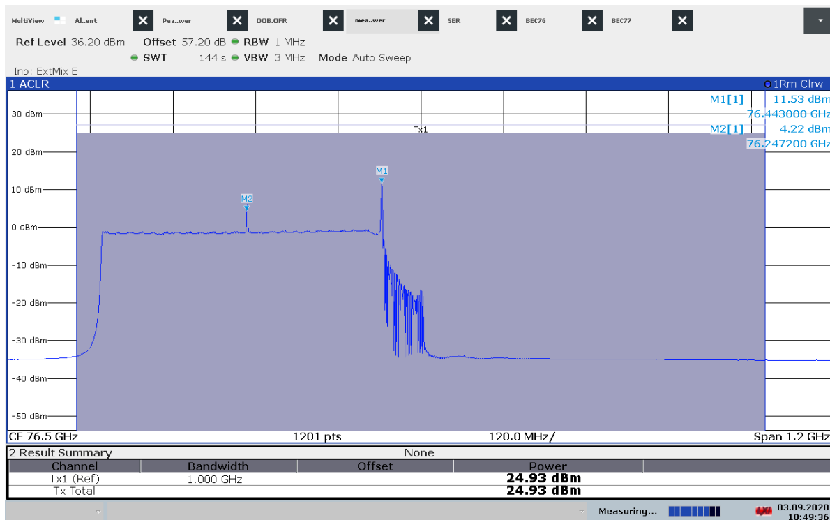
Plot 2: Mode 9(b), Radiated mean power, T_{nom} / V_{nom}
