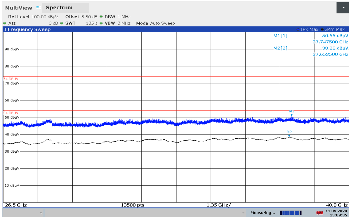
Plot 11: 26.5 GHz to 40 GHz, Mode 9(b)
