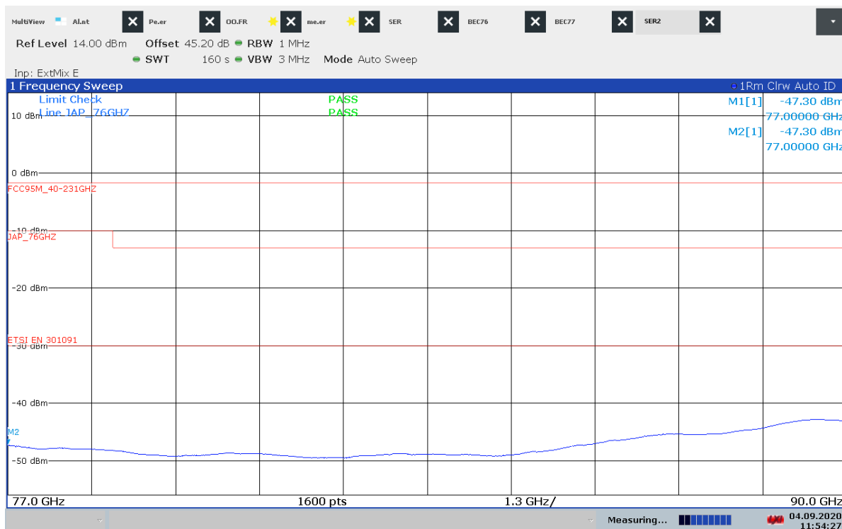
Plot 15: 77 GHz to 90 GHz, Mode 9(b)
