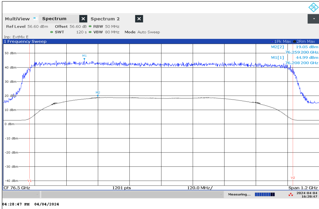
Plot 1: EIRP Peak Power, Mode 03, Peak detector, T_{nom} / V_{nom}
