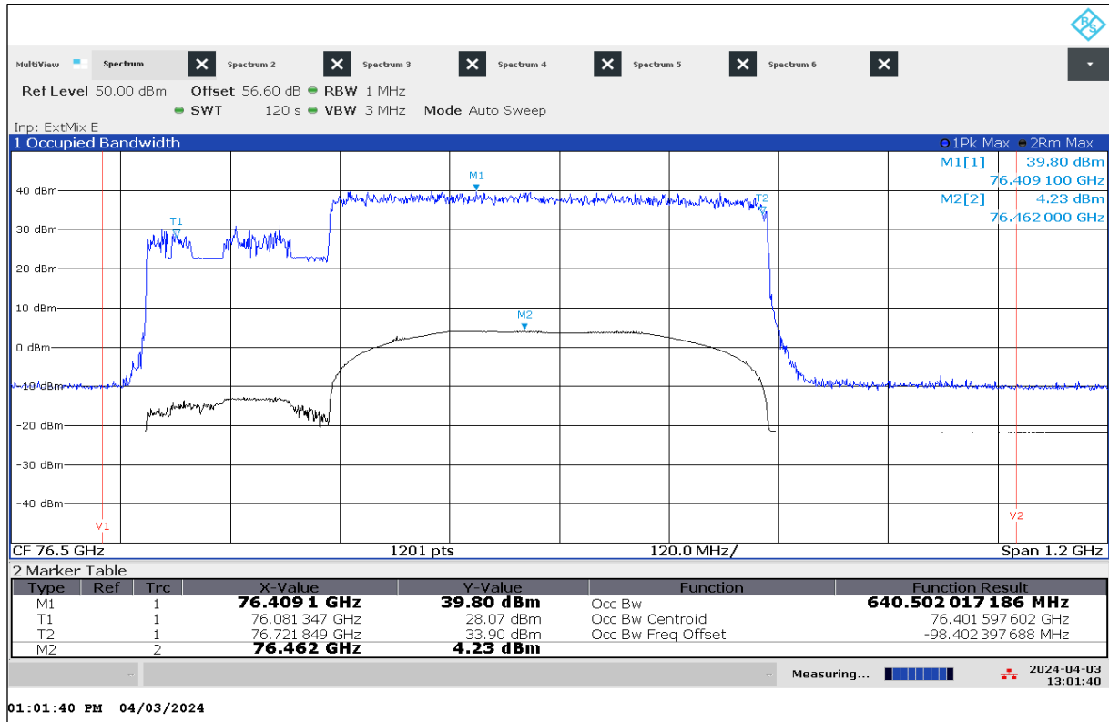
Plot 16: OBW, Mode 39, T_{nom} / V_{nom}
