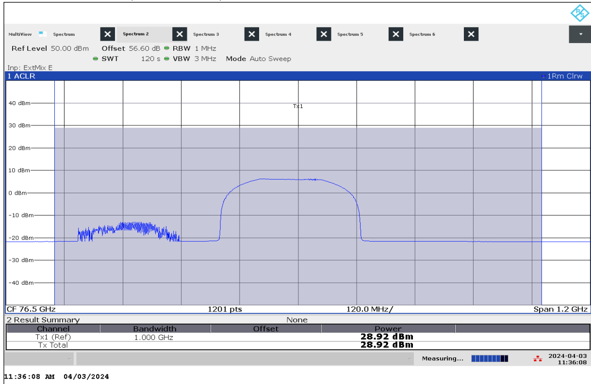
Plot 12: EIRP Mean Power (Channel Power), Mode 63, RMS detector, T_{nom} / V_{nom}
