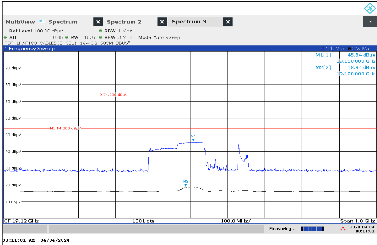
Plot 23: 19 GHz, Mode 63 (Worst case), antenna vertical / horizontal
