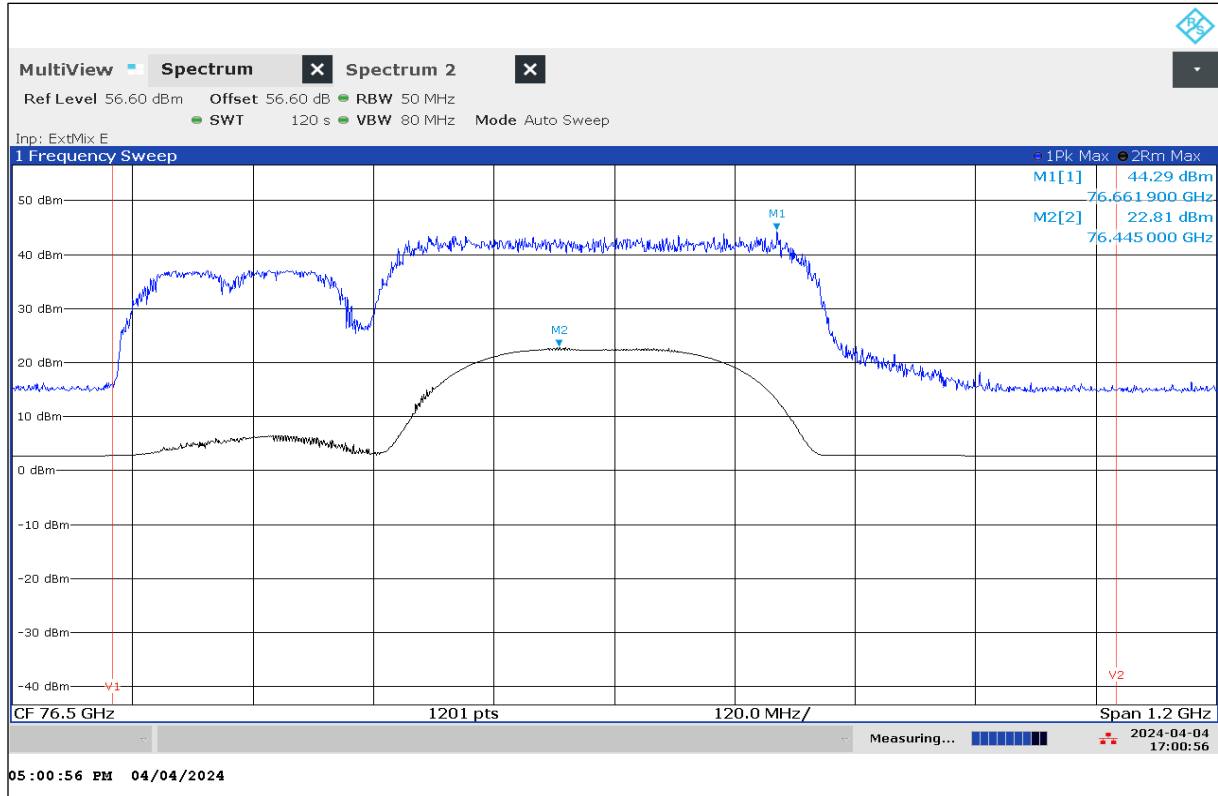
Plot 5: EIRP Peak Power, Mode 51, Peak detector, T_{nom} / V_{nom}
