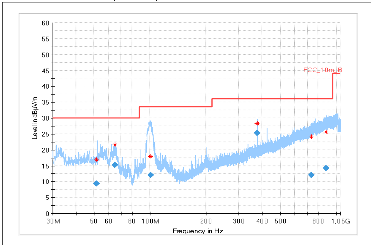
Plot 20: 30 MHz – 1 GHz, Mode 63 (Worst case), antenna vertical / horizontal
