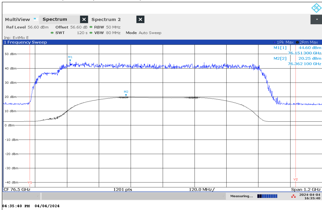
Plot 2: EIRP Peak Power, Mode 15, Peak detector, T_{nom} / V_{nom}
