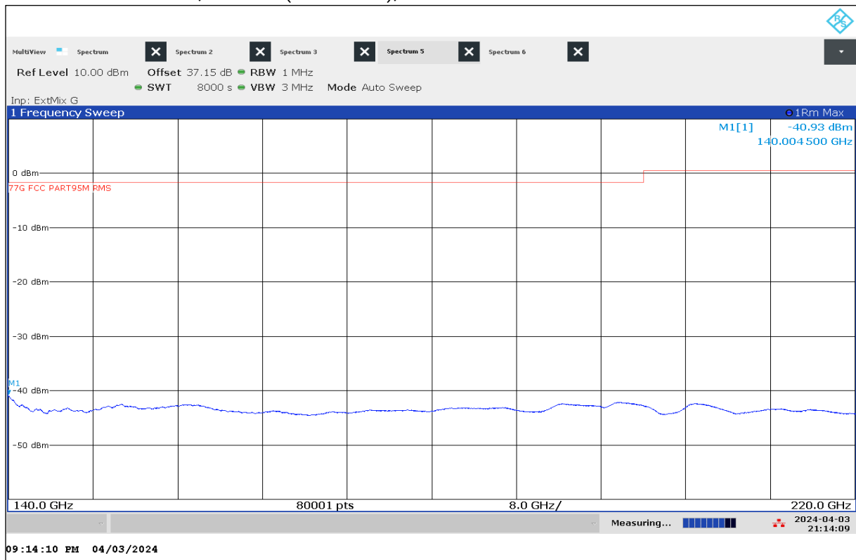
Plot 31: 140 GHz – 220 GHz, Mode 63 (Worst Case), antenna vertical / horizontal
