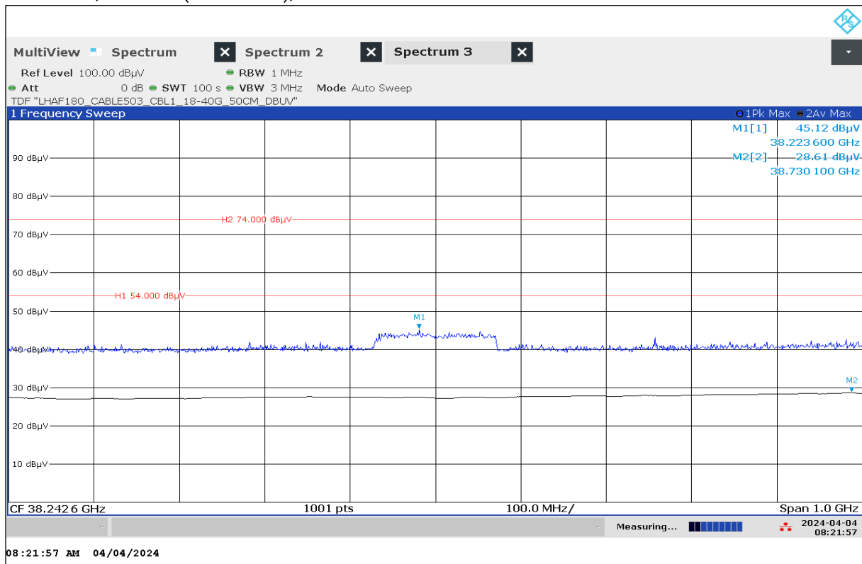
Plot 25: 38 GHz, Mode 63 (Worst case), antenna vertical / horizontal
