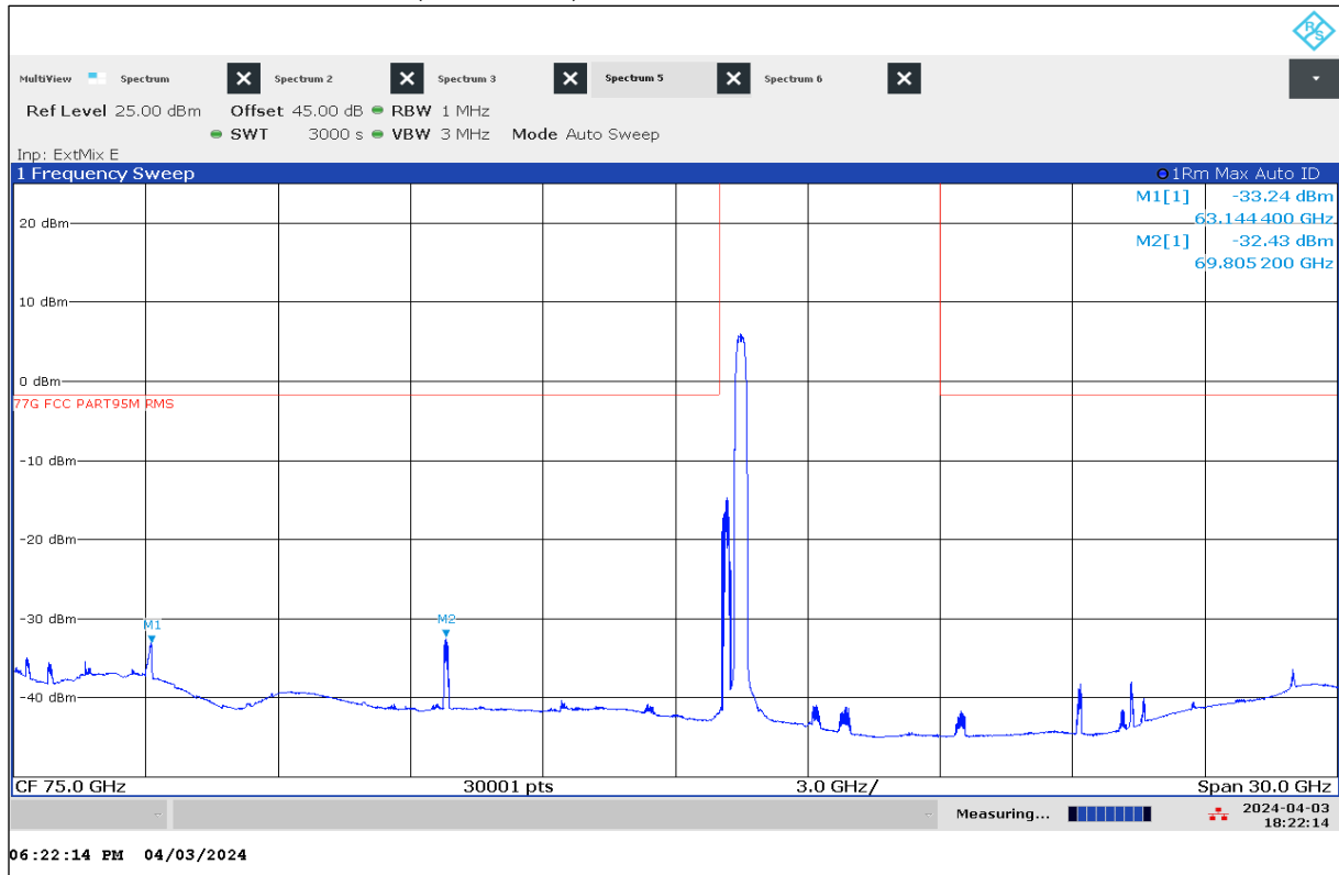
Marker show mixer products produced by harmonic mixer
