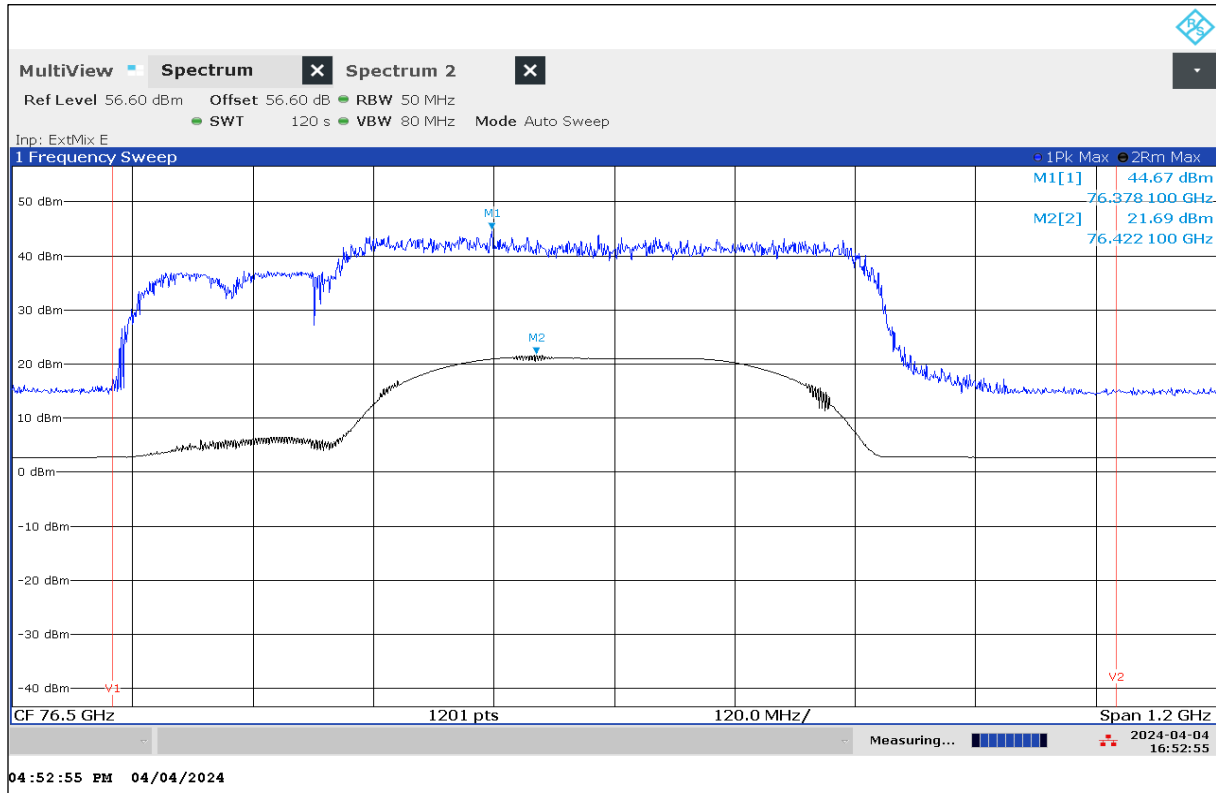
Plot 4: EIRP Peak Power, Mode 39, Peak detector, T_{nom} / V_{nom}
