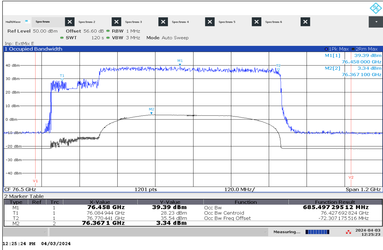
Plot 15: OBW, Mode 27, T_{nom} / V_{nom}
