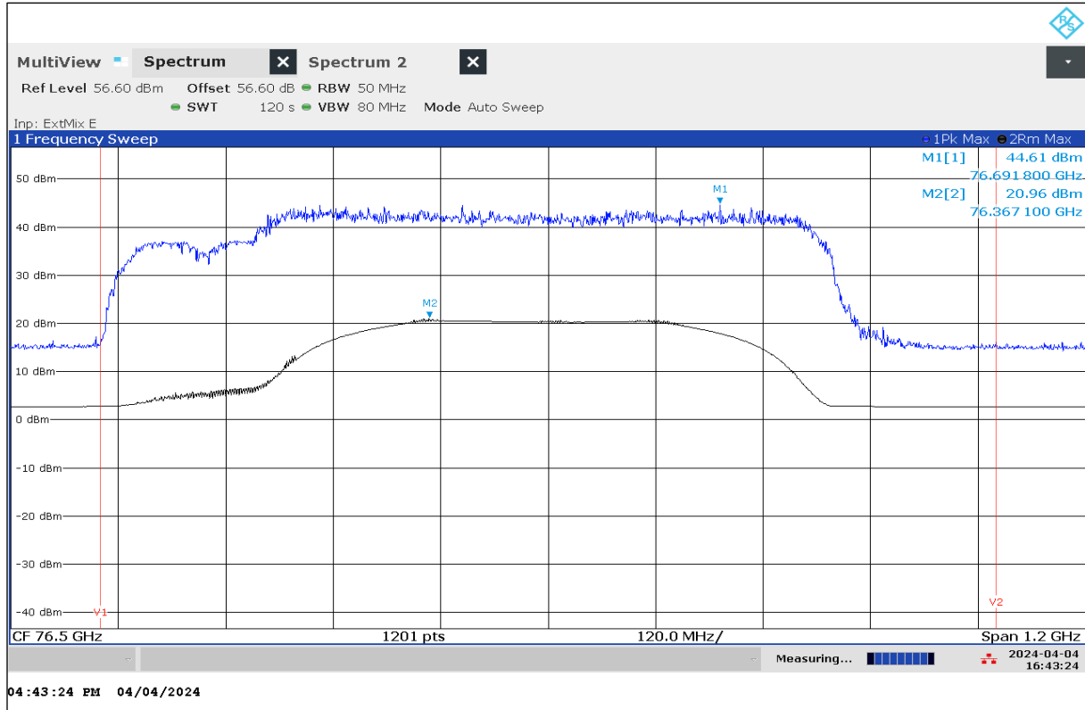
Plot 3: EIRP Peak Power, Mode 27, Peak detector, T_{nom} / V_{nom}
