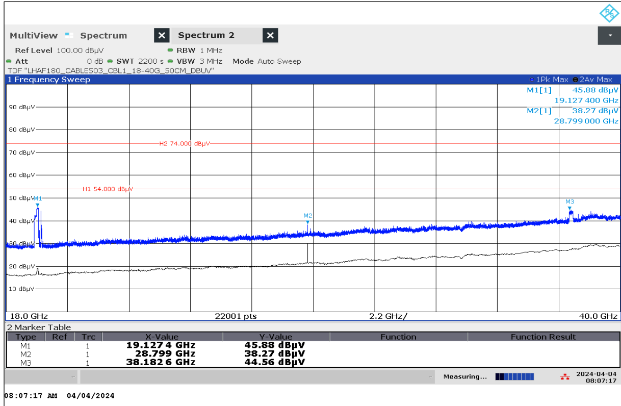
Plot 22: 18 GHz – 40 GHz, Mode 63 (Worst Case), antenna vertical / horizontal
