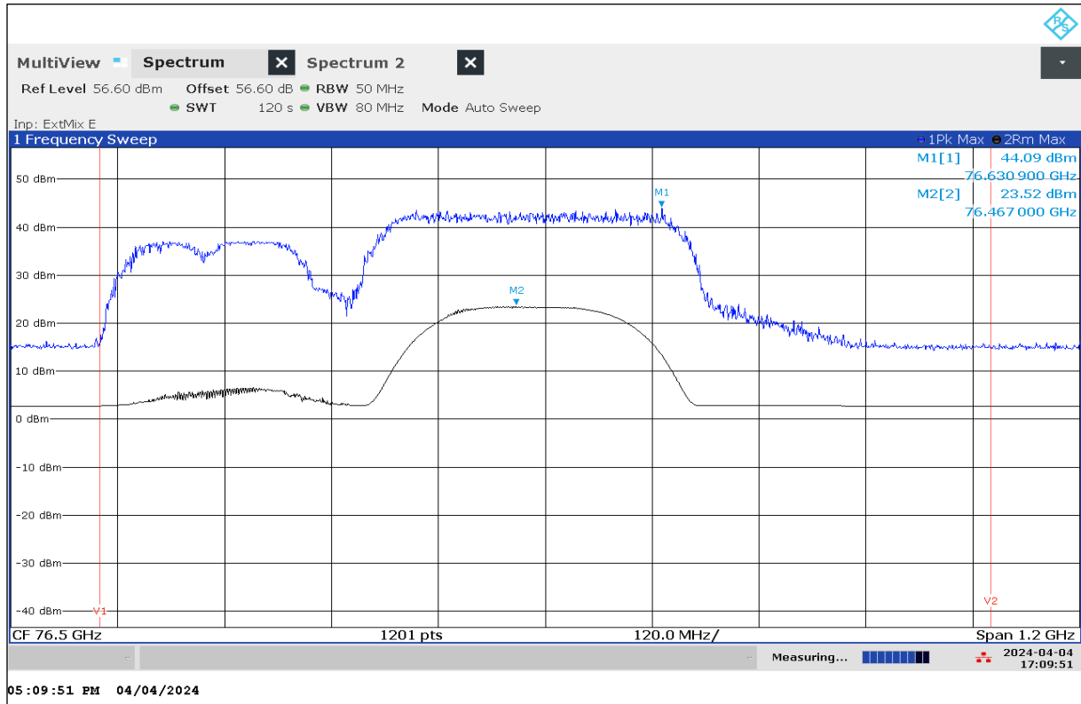
Plot 6: EIRP Peak Power, Mode 63, Peak detector, T_{nom} / V_{nom}
