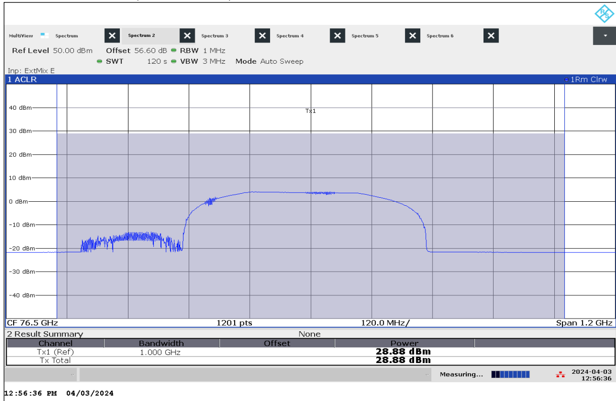
Plot 10: EIRP Mean Power (Channel Power), Mode 39, RMS detector, T_{nom} / V_{nom}
