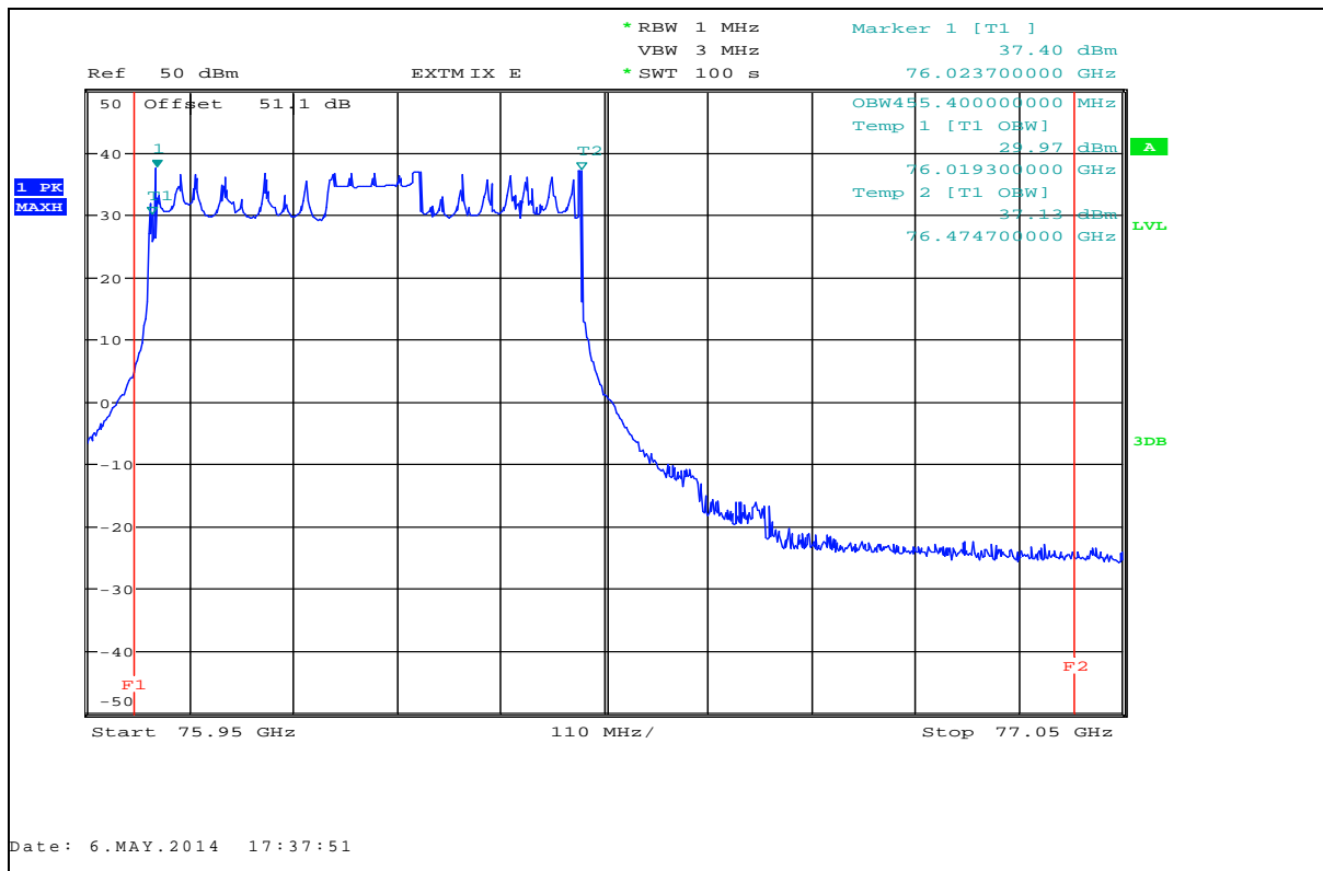
Plot 22: Occupied bandwidth (99%), T_{nom} / V_{nom} , mid frequency
