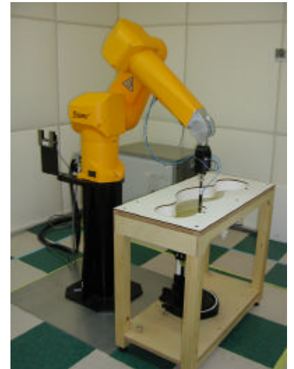
Figure 1. SAR System
