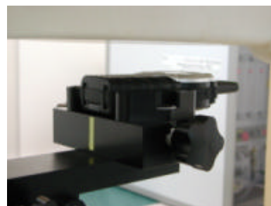
Figure 11. Mouth Face SAR Test Setup
