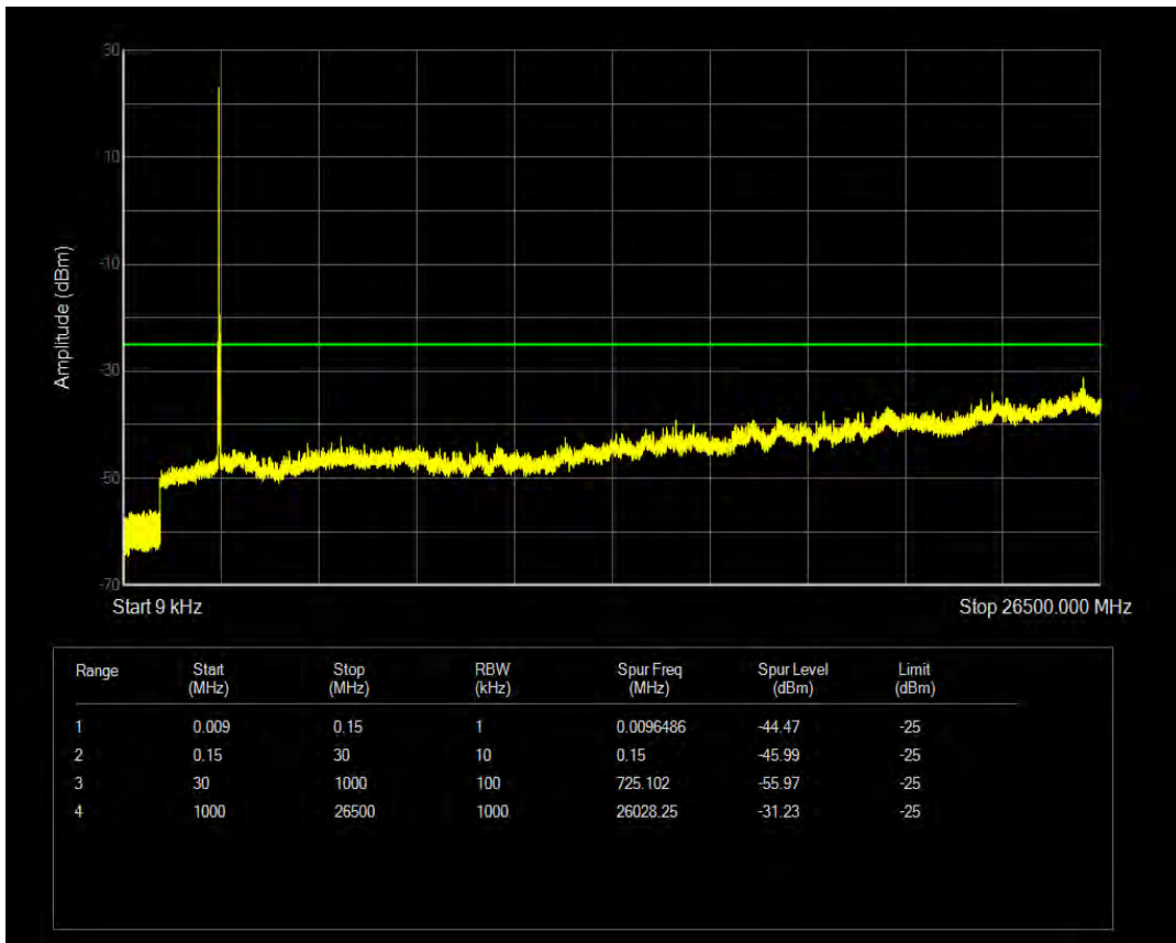
Band41 16QAM BW=15MHz Channel=41365 RB Size=75 Position=#0
