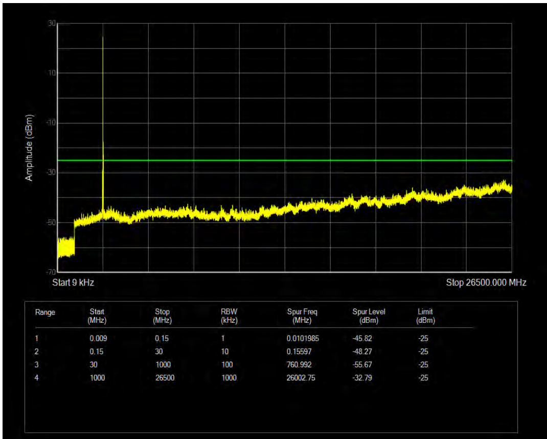
Band41 16QAM BW=15MHz Channel=40115 RB Size=75 Position=#0
