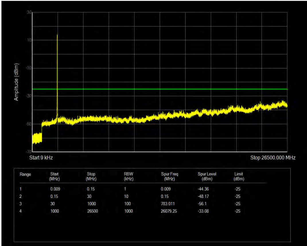
Band41 QPSK BW=20MHz Channel=41340 RB Size=1 Position=#0
