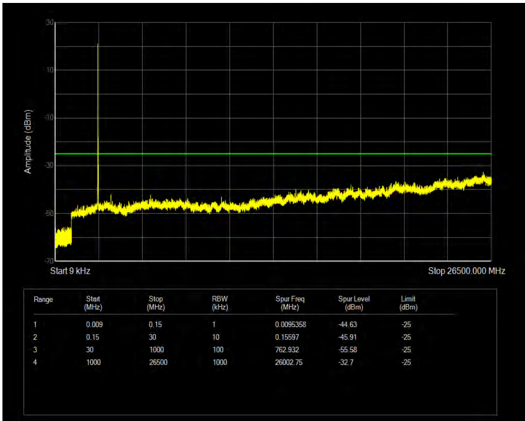
Band41 16QAM BW=20MHz Channel=40140 RB Size=100 Position=#0
