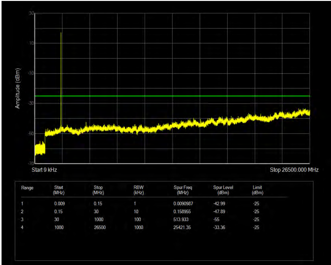
Band41 16QAM BW=20MHz Channel=41340 RB Size=1 Position=#0
