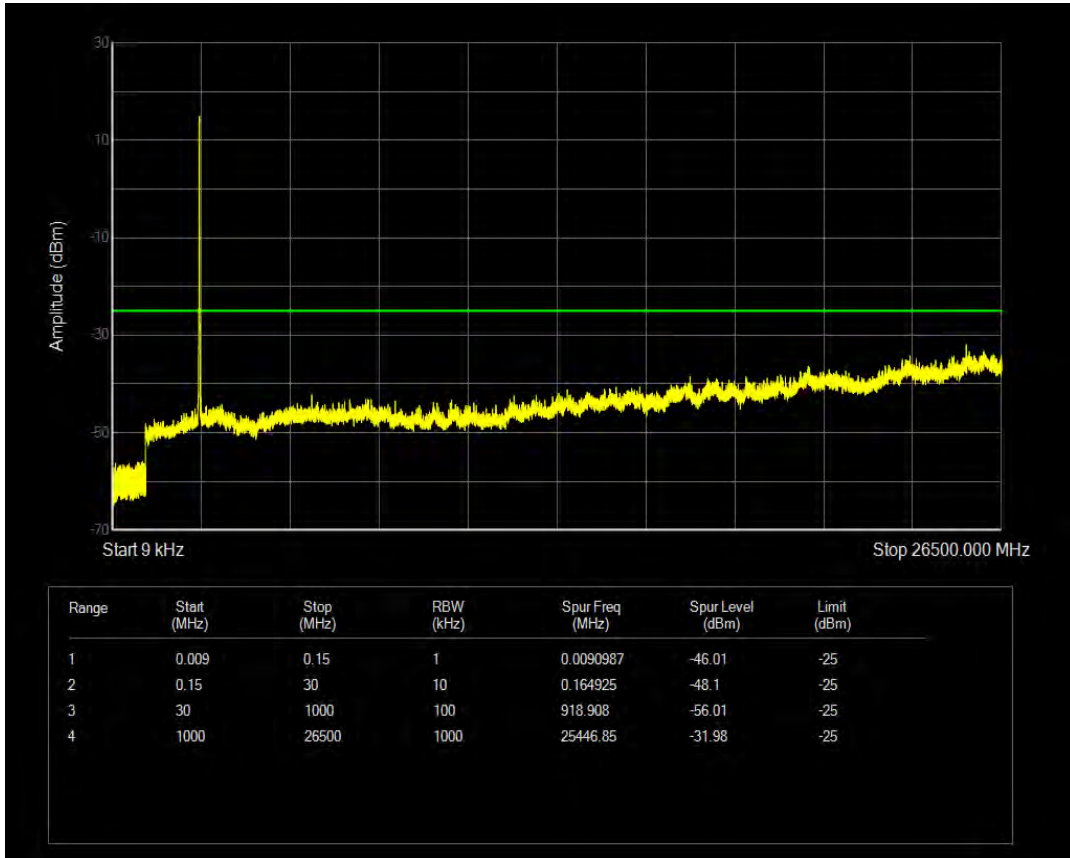
Band41 QPSK BW=15MHz Channel=41365 RB Size=1 Position=#0
