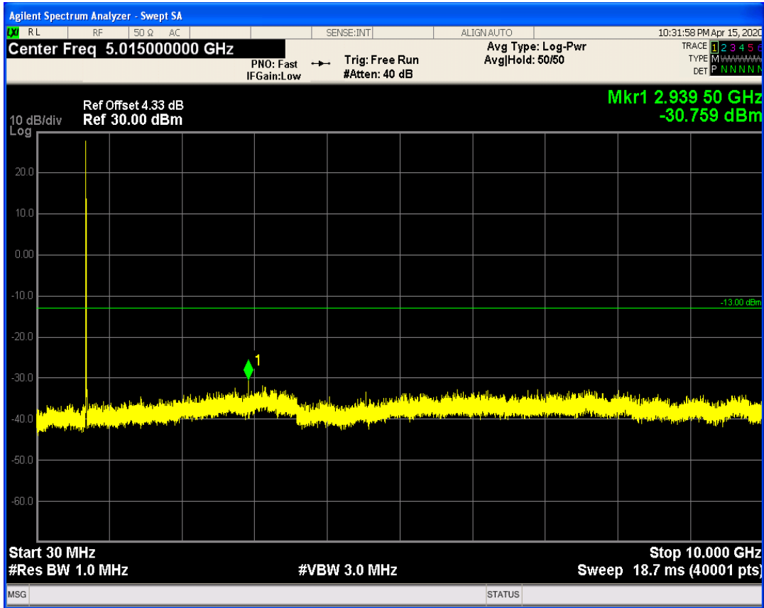
LTE Band13 QPSK BW=5MHz Channel=23205 RB Size=25 Position=#0
