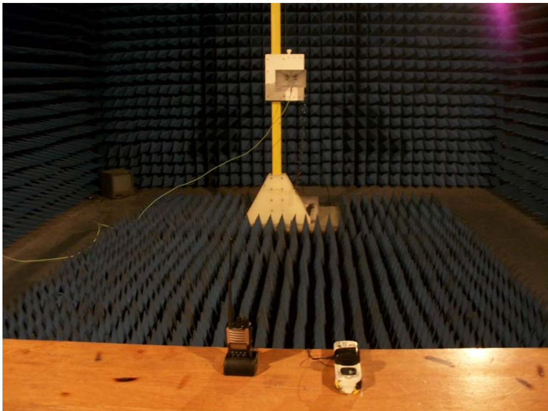
Radiated spurious Emission setup 1(Above 1GHz)
