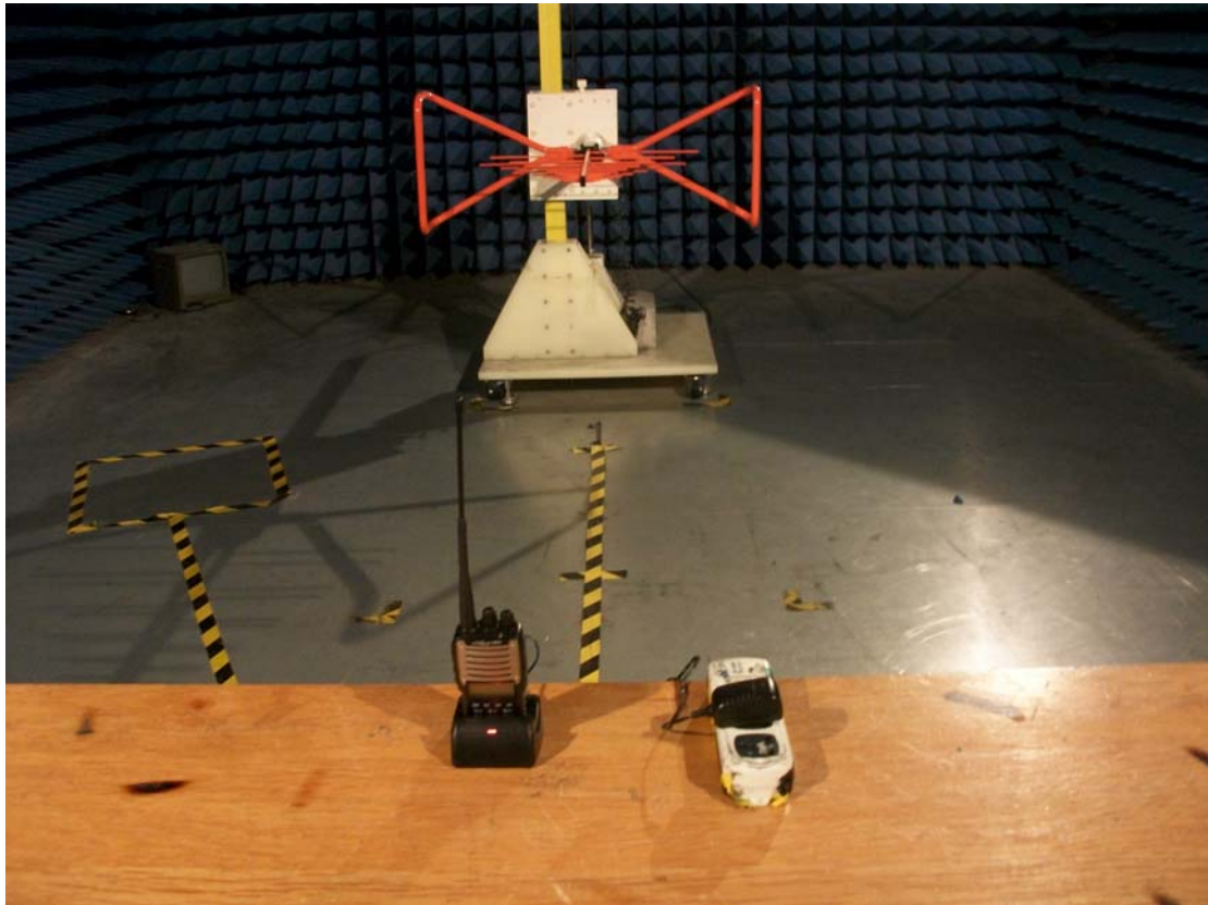
Radiated spurious Emission setup 1(Below 1GHz)
