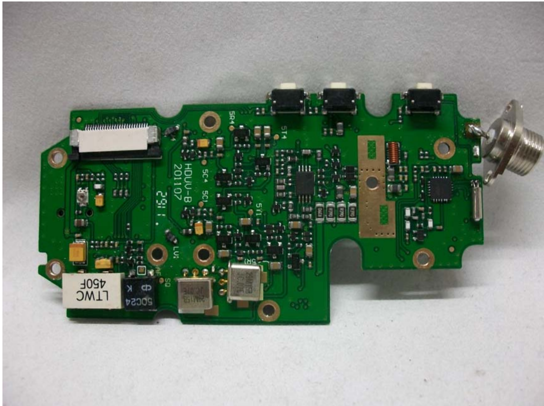
Solder Board – Component View 3
