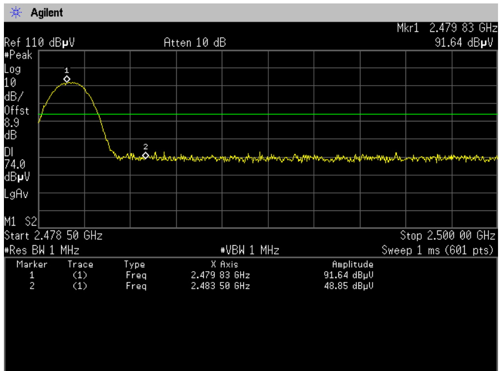
(8-DPSK CH High, Vertical, Peak)
