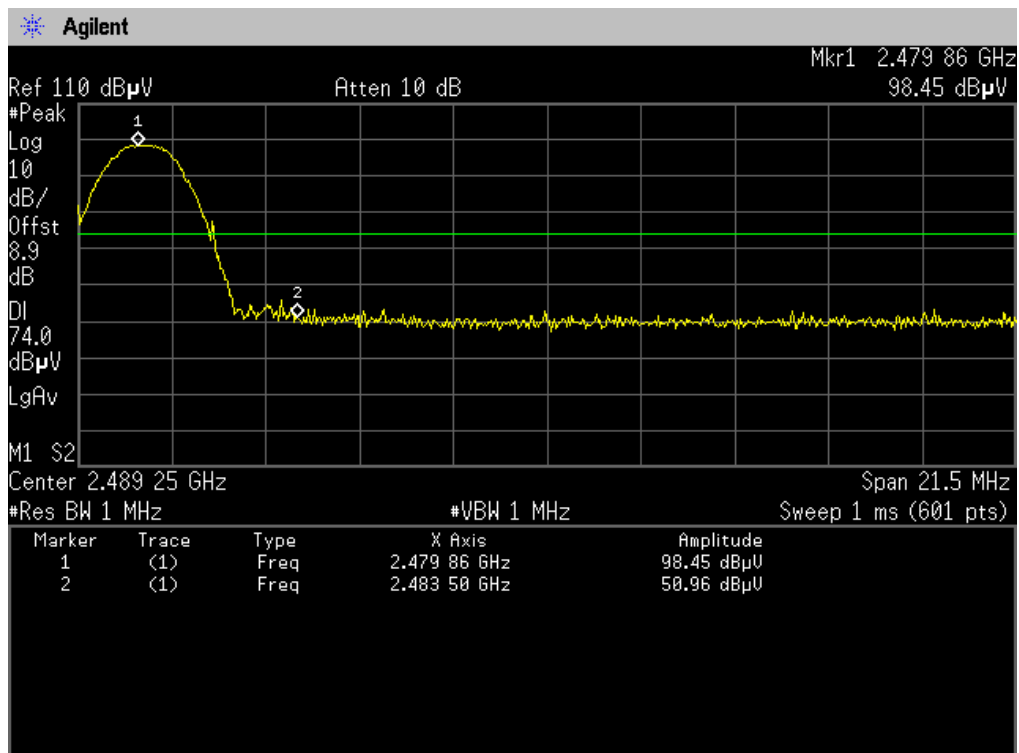
(8-DPSK CH High, Horizontal, Peak)
