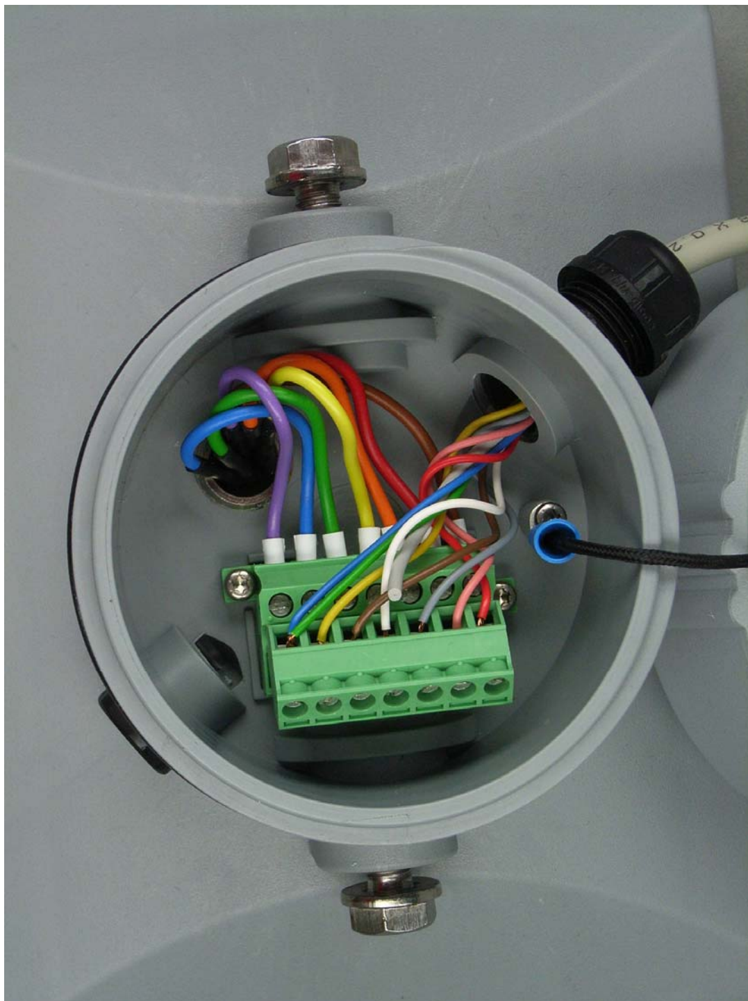
71069_e.jpg RLS, rear housing opened
