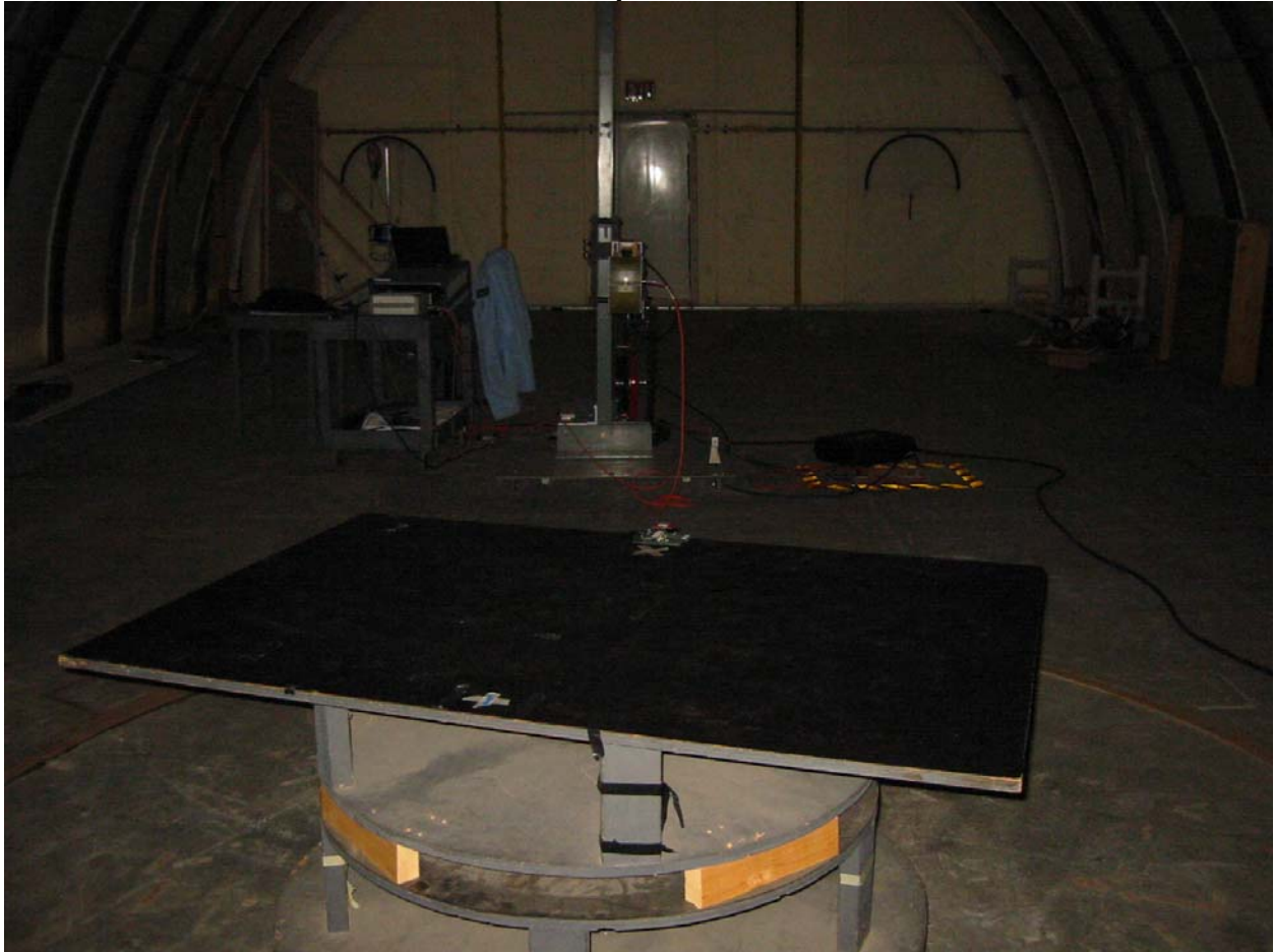
Radiated Emissions, 1-4 GHz
