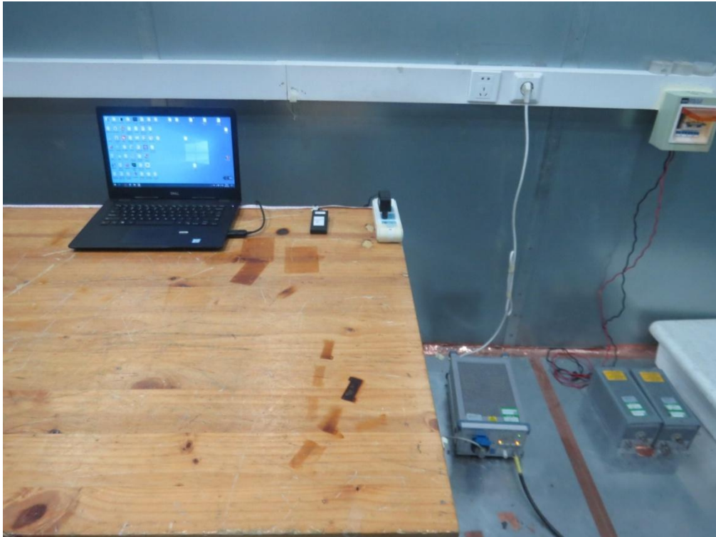
Picture 1: Conducted Emissions Test Setup
