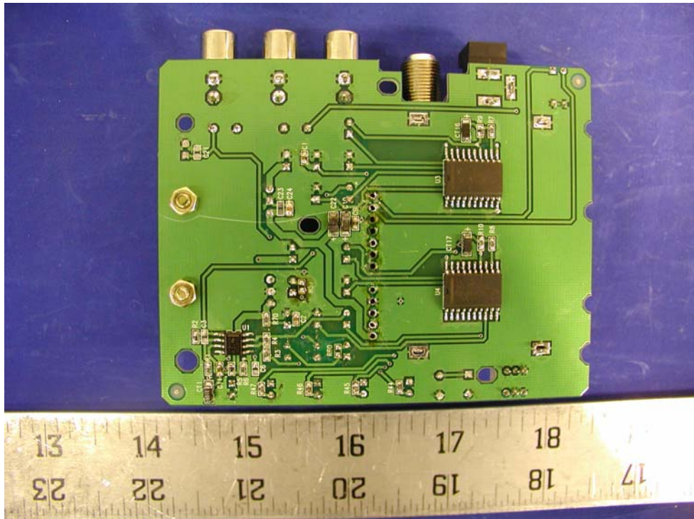
Main Board - Solder View
