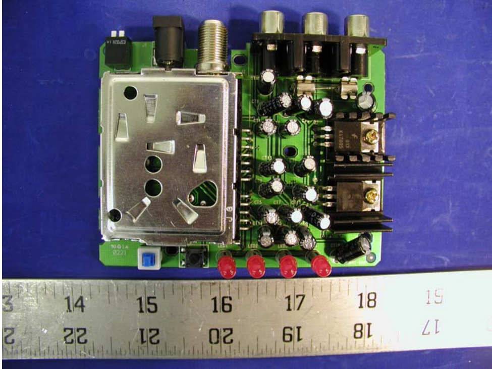
Main Board - Component View
