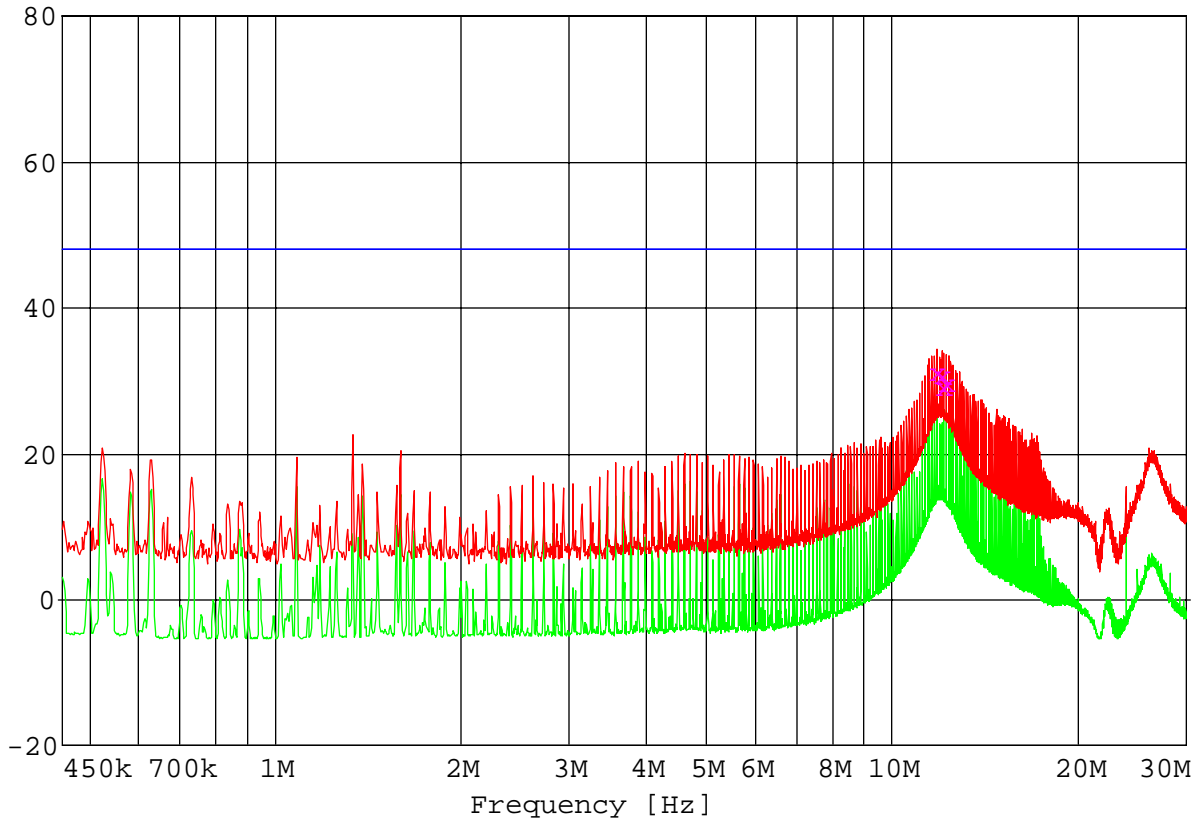
Quasi-Peak Measurements
