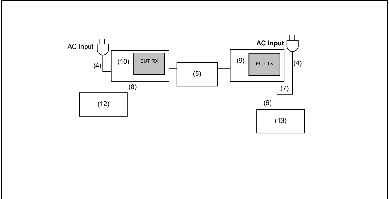
Conduction Emission & Radiated Emission (Below 1 GHz)
