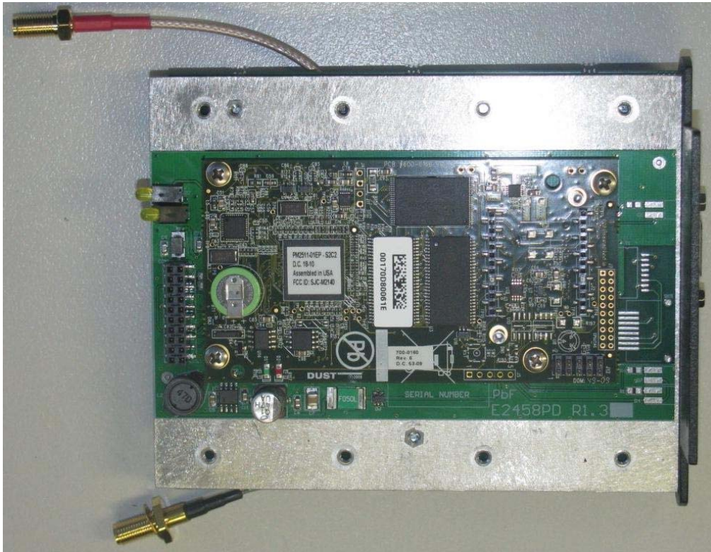
Main rear board with both Wi Hart radio module boards removed
