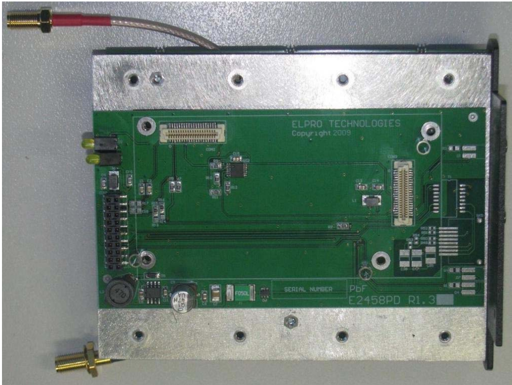
Main rear board with both Wi Hart radio module boards removed
