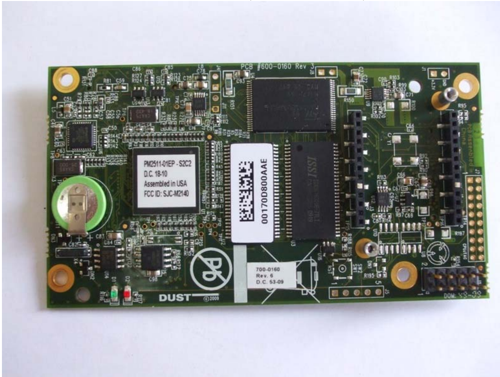
Front of the main Wi Hart radio module board (FCC ID: SJC-M2140).
