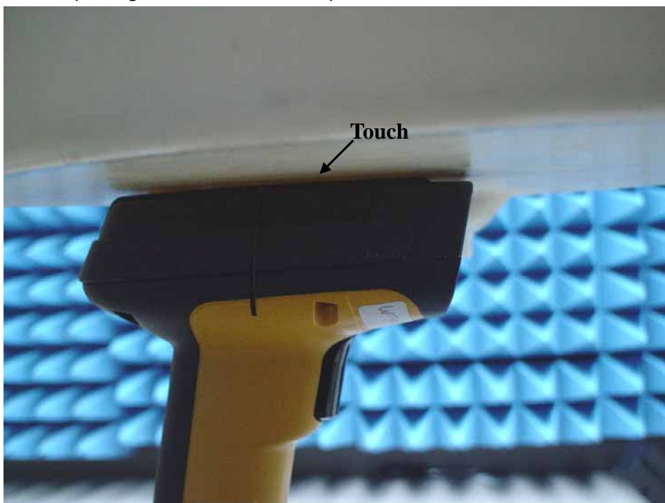
Fig.4 Photo of the EUT face-on contact to the Flat phantom, Spacing between EUT and phantom –In contact (0mm)
