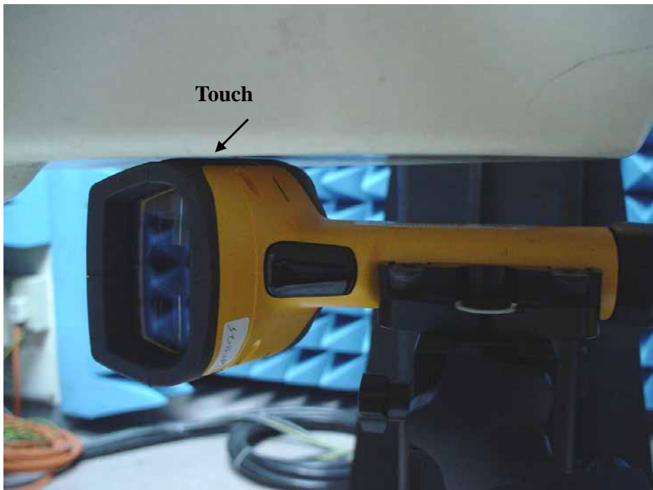
Fig.6 Photo of the EUT Left-side contact to the Flat phantom, Spacing between EUT and phantom –In contact (0mm)
