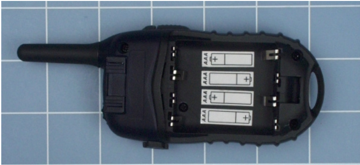
Battery Compartment
