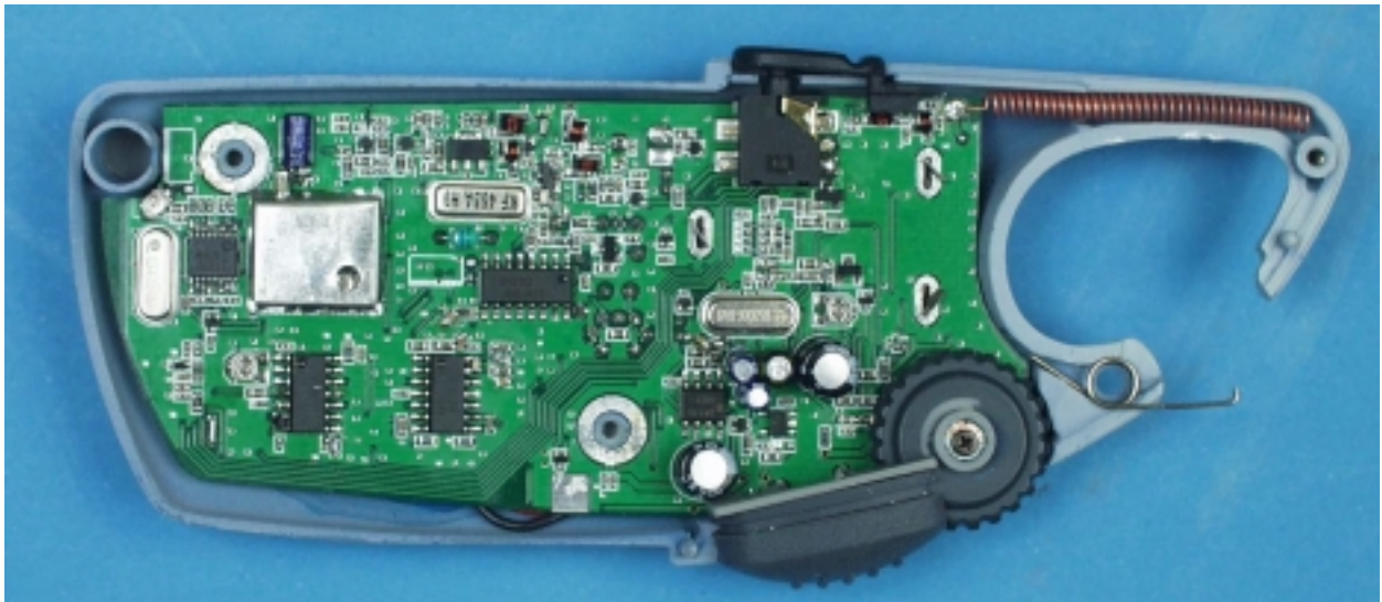
PCB Component Side
