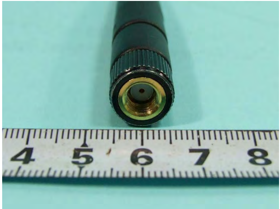
Omni-Direction Antenna (S24513BPX)
