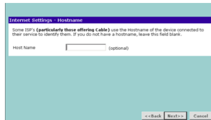
Figure 18 Hostname Screen
