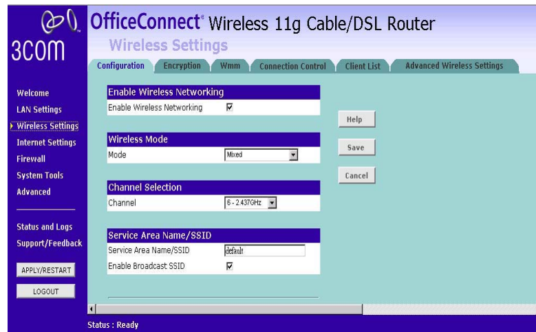
Figure 34 Configuration Screen
