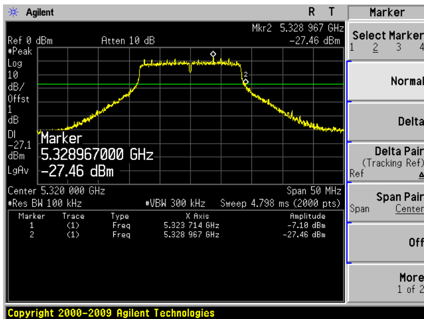
Channel 64 (5320MHz)
