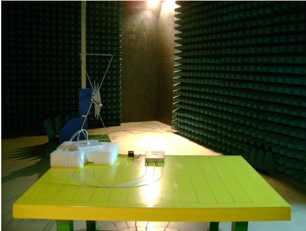
Radiated Emission Test set-up photo (Antenna 5)
