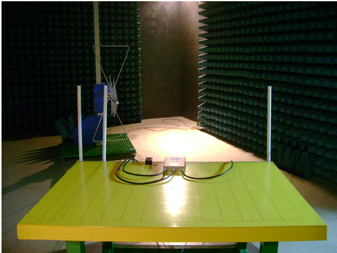
Radiated Emission Test set-up photo (Antenna 2)
