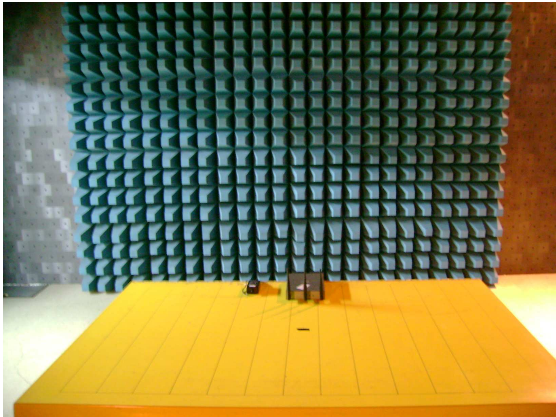
Radiated Emission Test set-up photo (Antenna 1)
