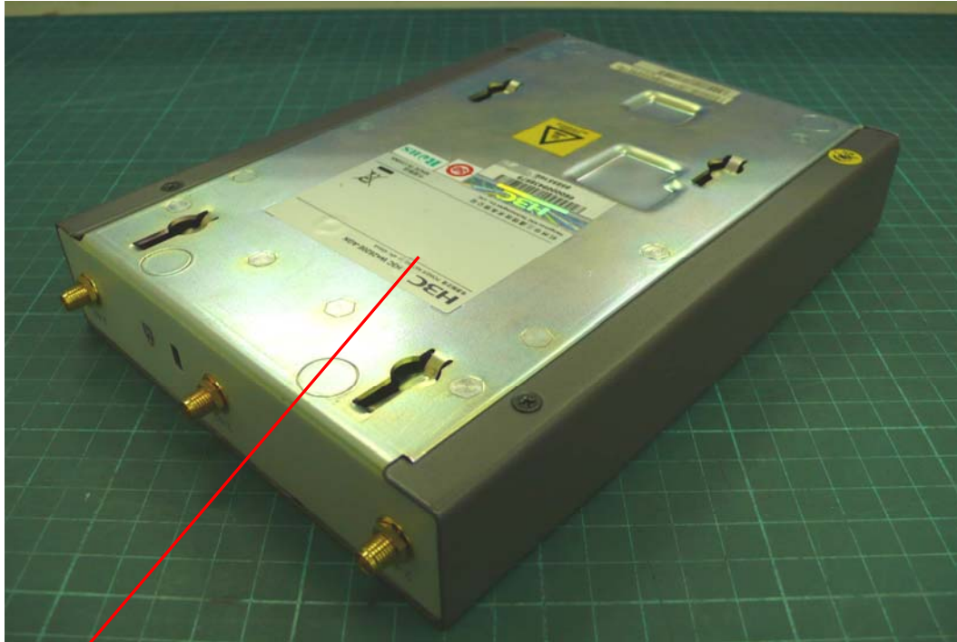
FCC ID & IC Label Location
