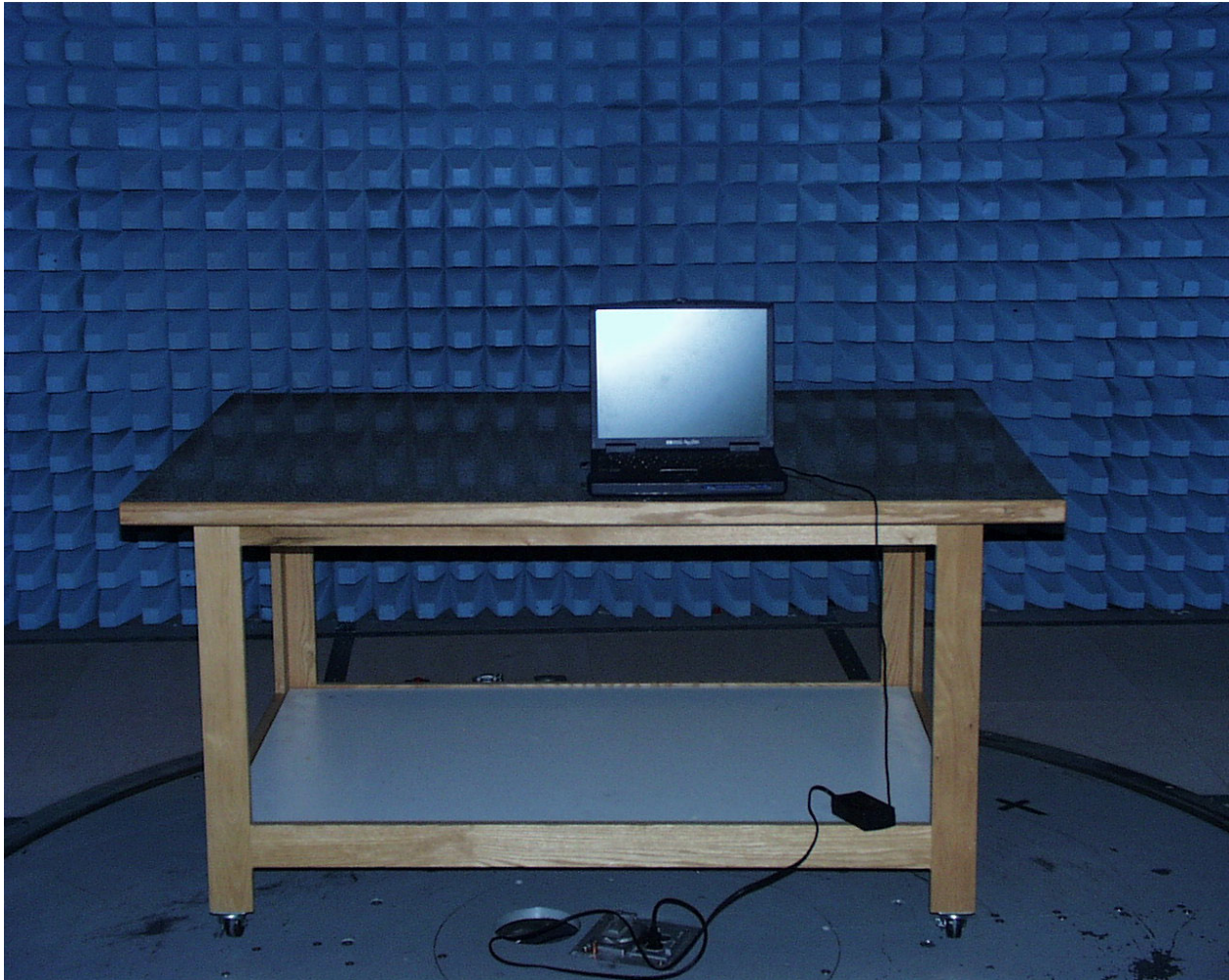
Front view SL-1110 Retractable Antenna radiated emissions Test Setup
