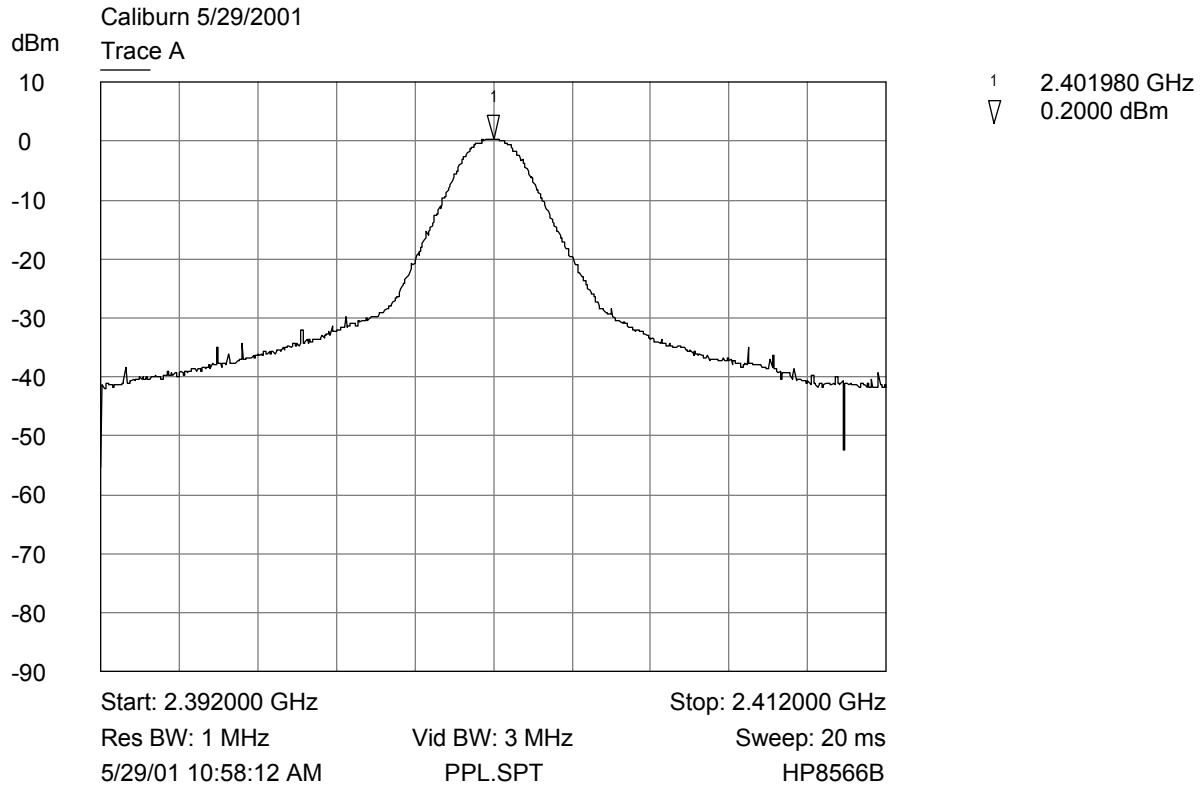
Peak Output Power Plot - (Low Channel)
