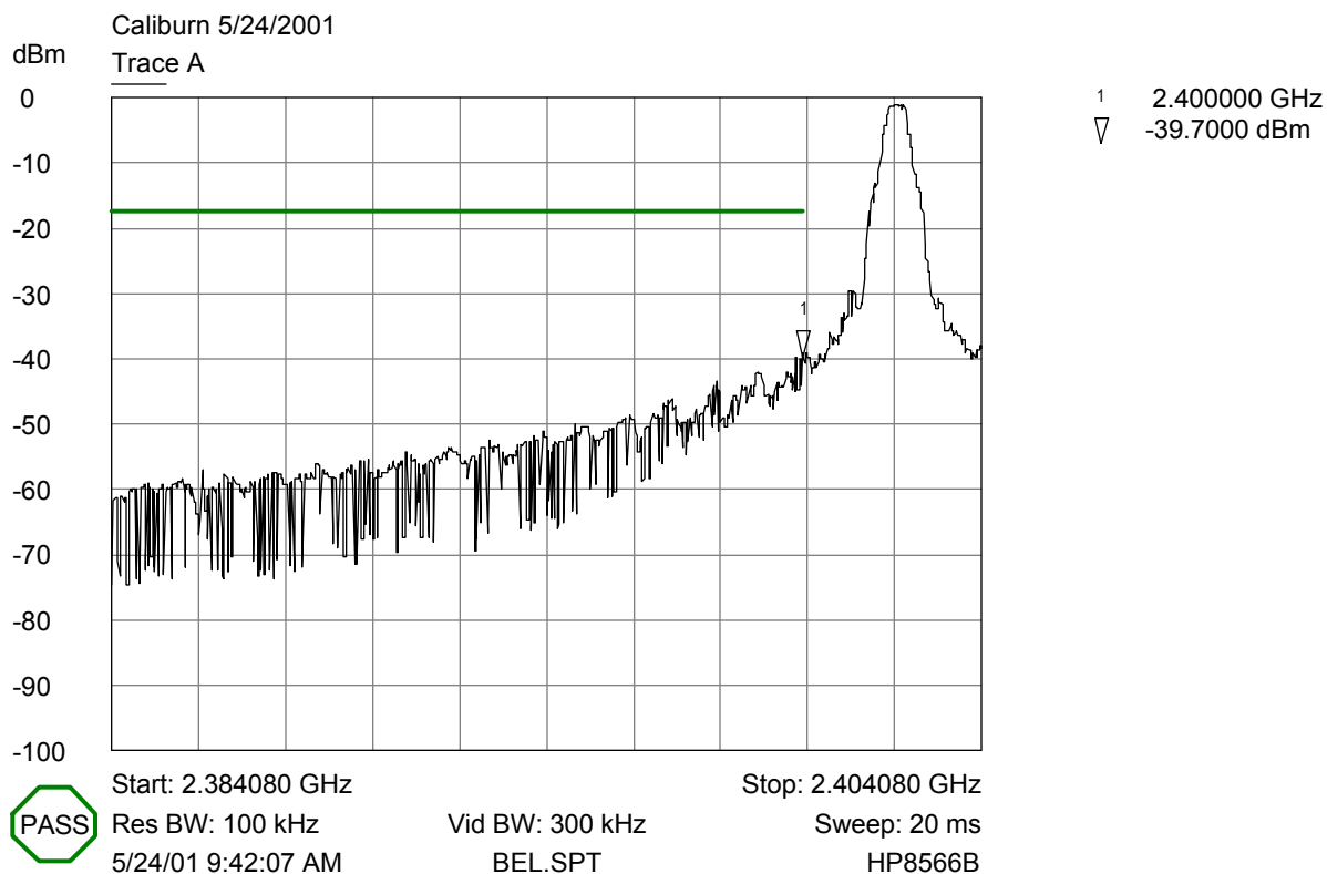
Band Edge Plot, 2402 MHz
