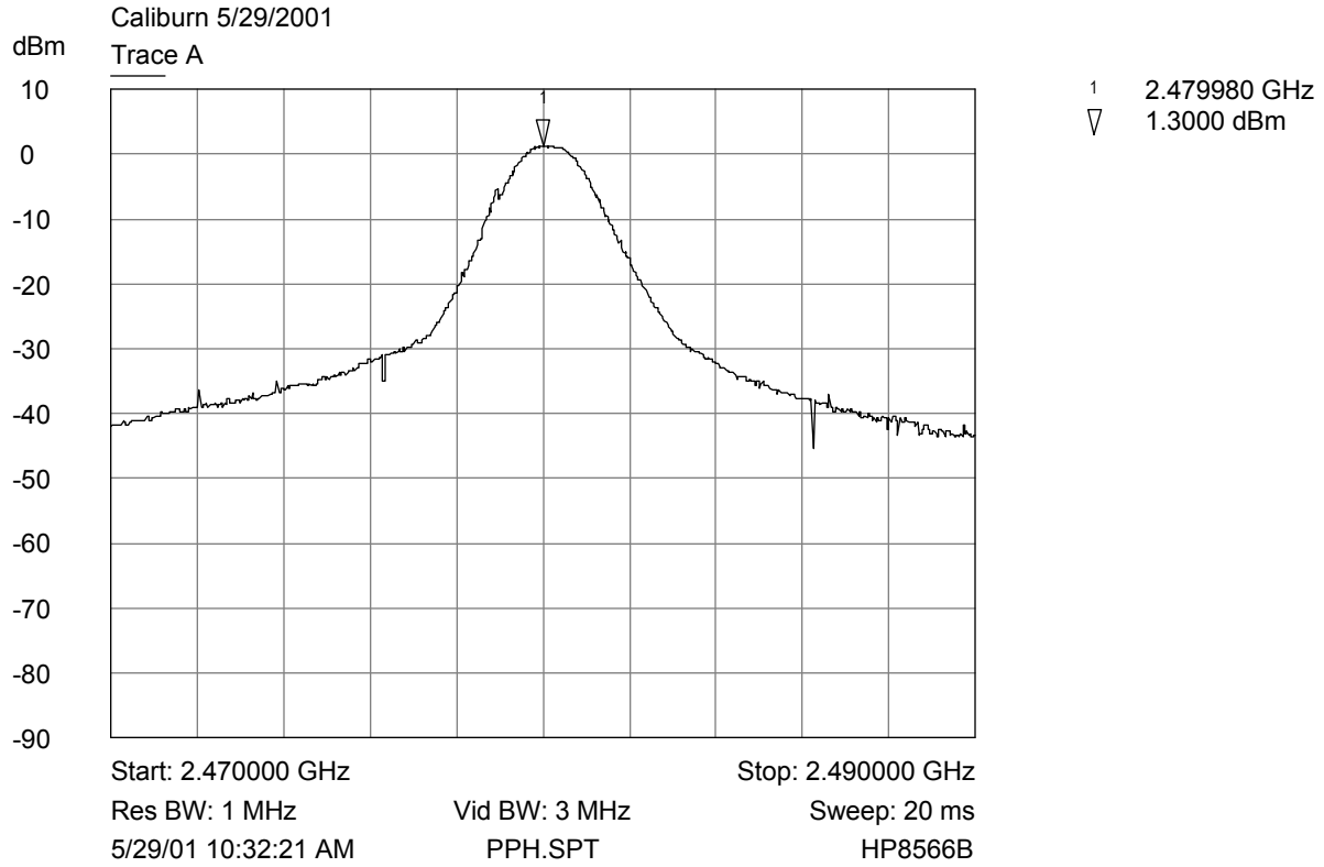
Peak Output Power Plot - (High Channel)
