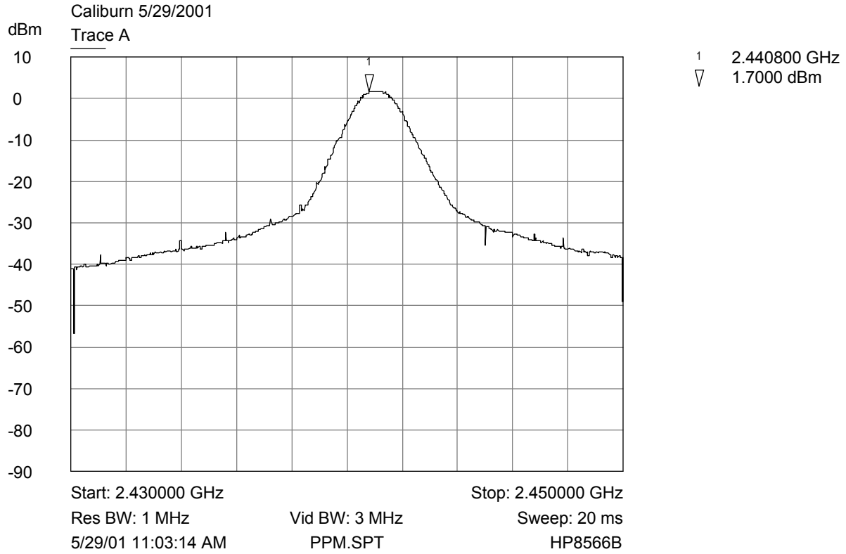
Peak Output Power Plot - (Middle Channel)
