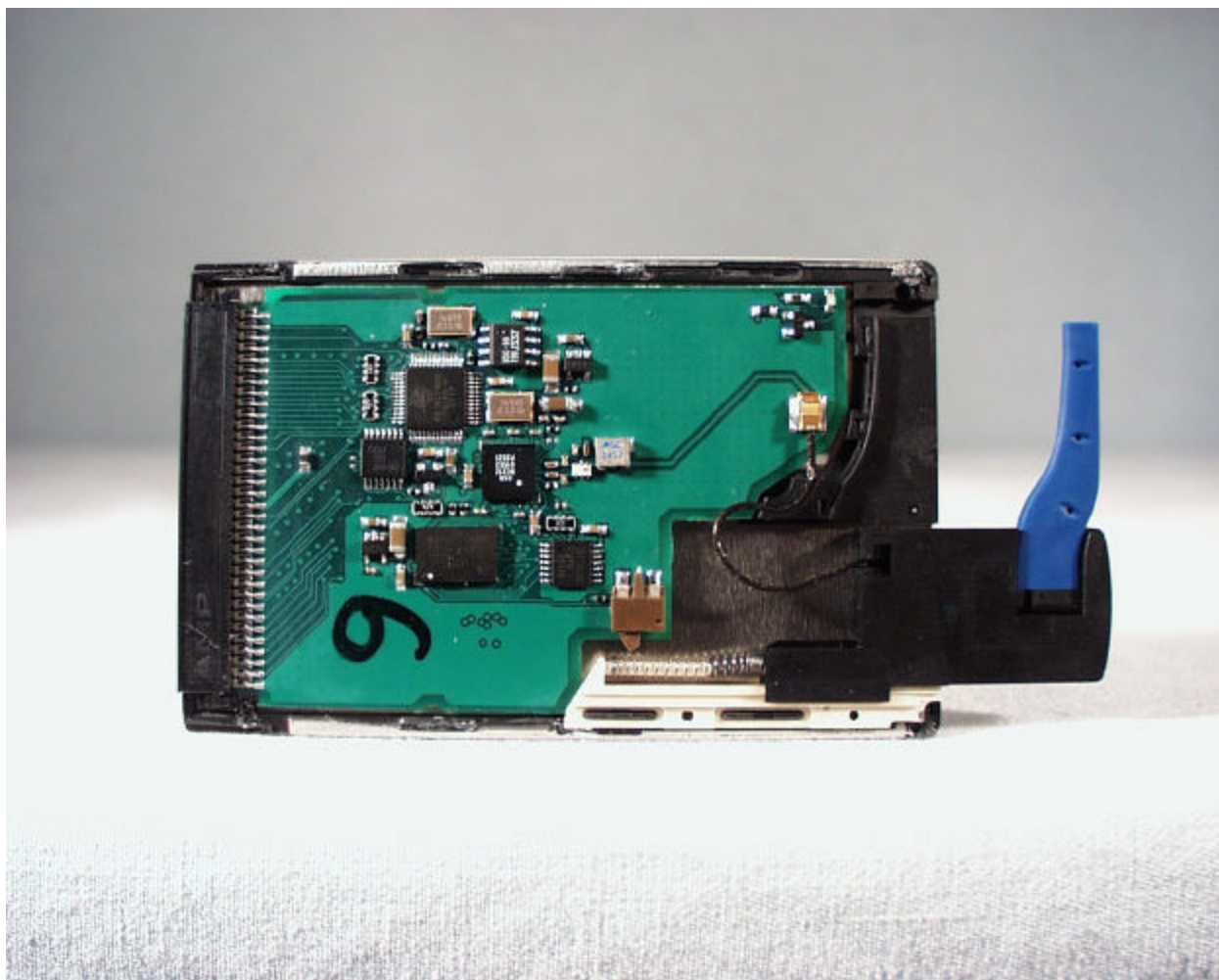
Component Side of the SL-1022 PCB
