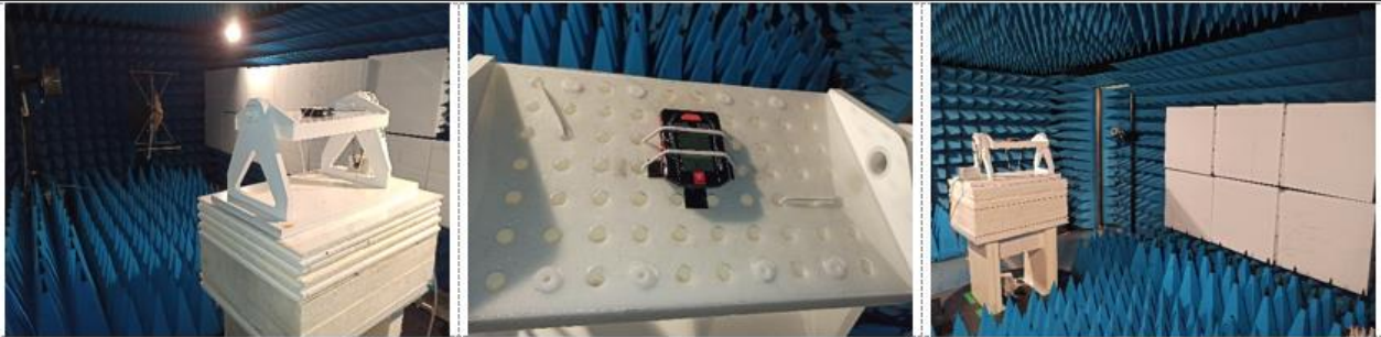
Photo Setup : anechoic chamber (XY axis)
