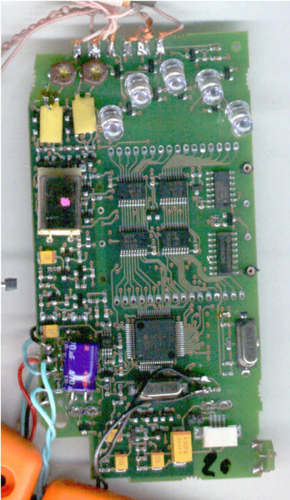
Components side (front face)
