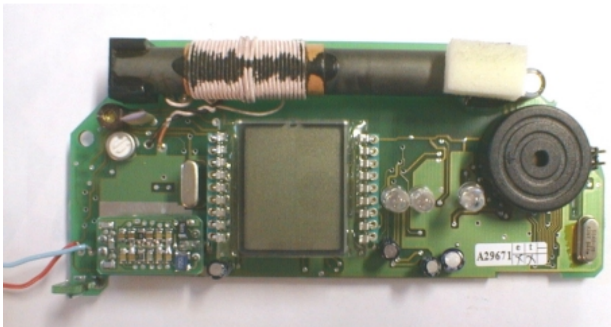
2 – Internal board, upper face (small metallic cover removed)
