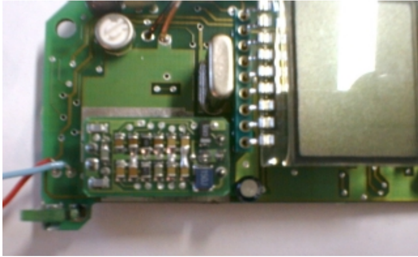
3 – Internal board, detail
