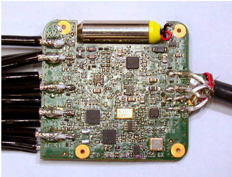
Photograph No. 8 Sensor array PCB second side view
