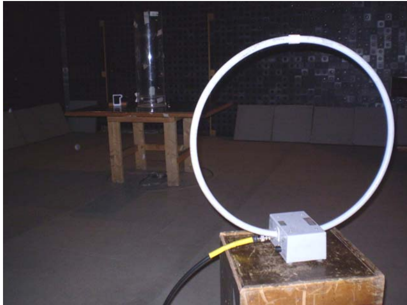
Photograph No.2 Out of band radiated emissions measurement setup with loop antenna in the anechoic chamber
