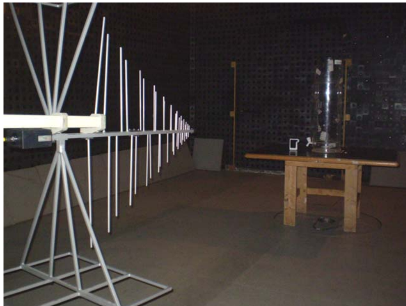
Photograph No.3 Out of band radiated emissions measurement setup in the anechoic chamber with biconilog antenna
