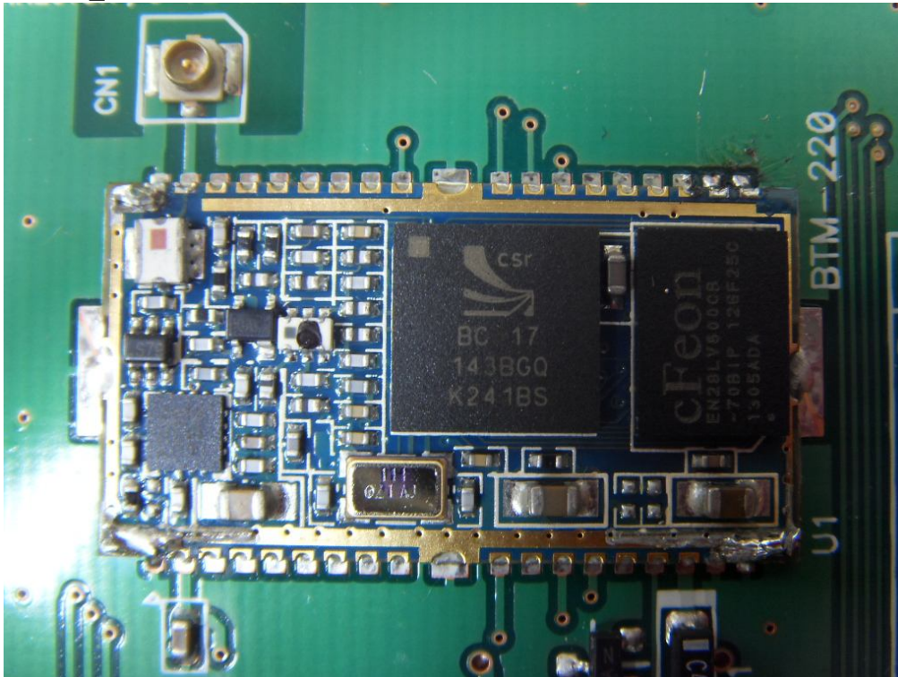
Antenna location
