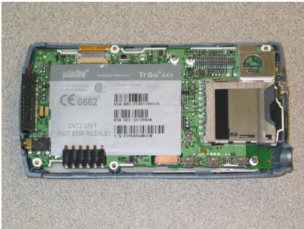
Main PCB, Label Side
