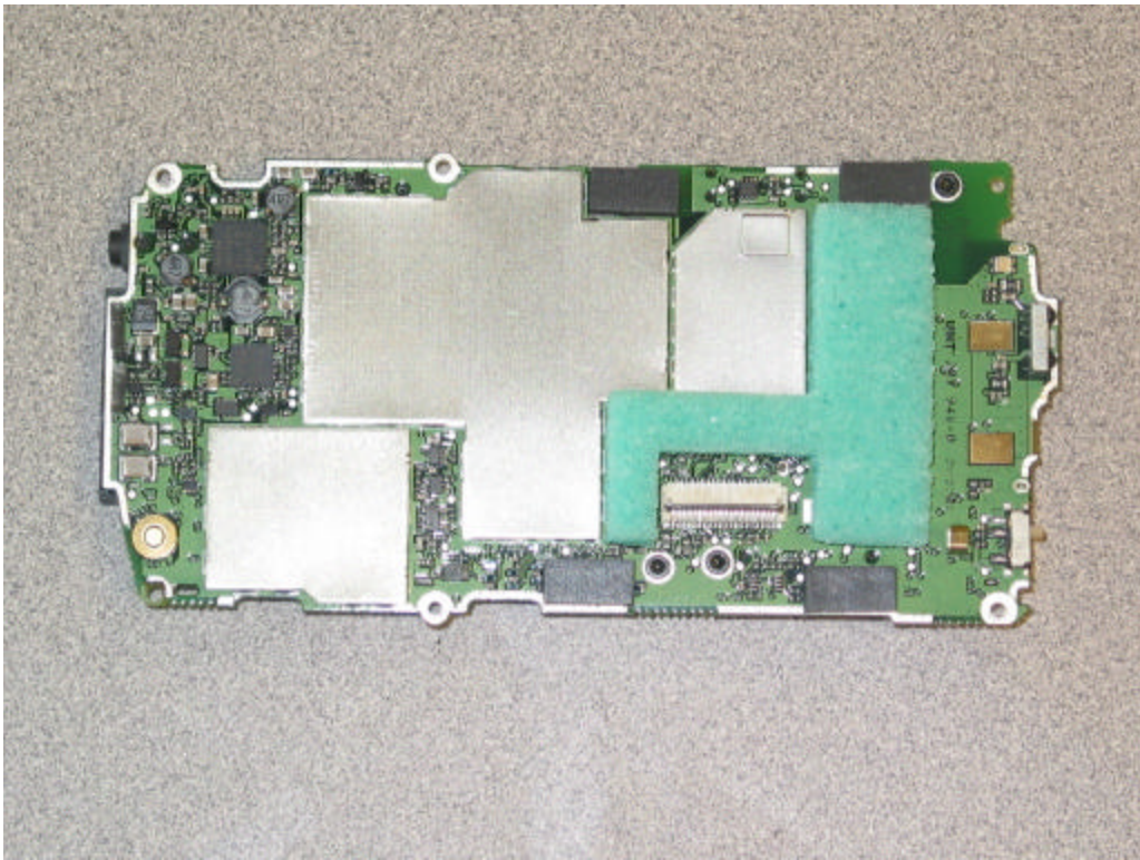
Main PCB , Shield Side
