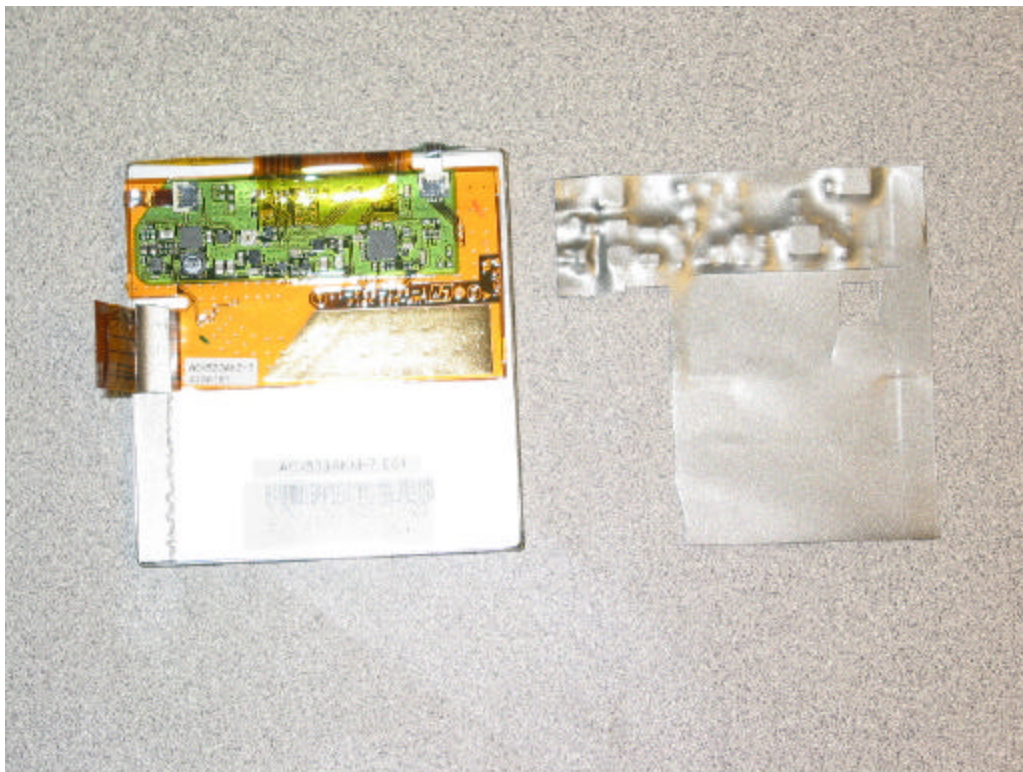
Display, Rear, Shield Removed
