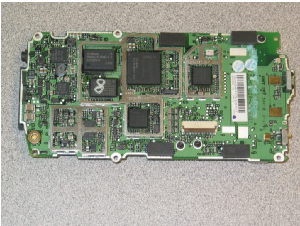
Main PCB, Shields Removed
