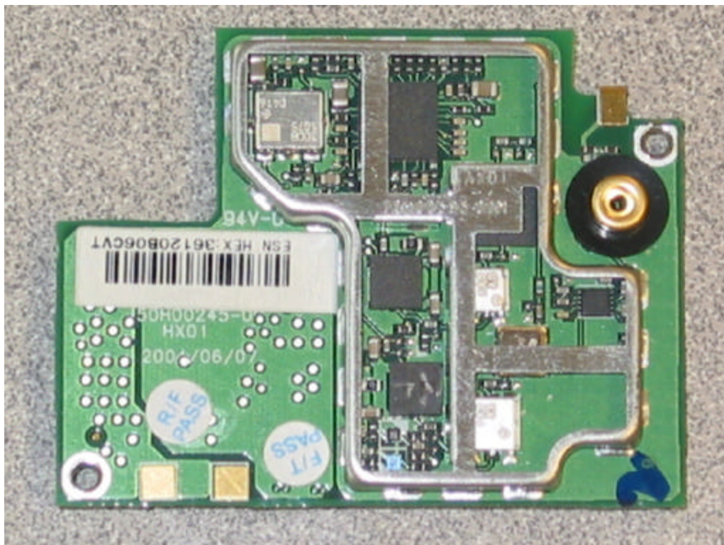
RF Moduel , Shields Removed
