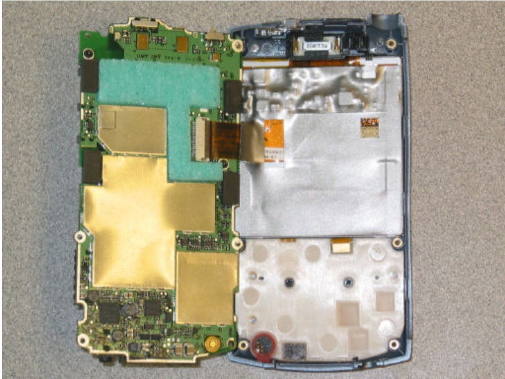
Main PCB / Keyboard & Display
