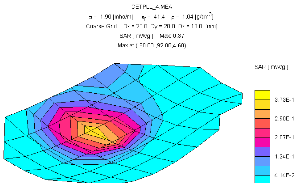
Fig. 5: SAR distribution plot with maximum local SAR value for PCS 1900 (channel 0512, left hand position).
