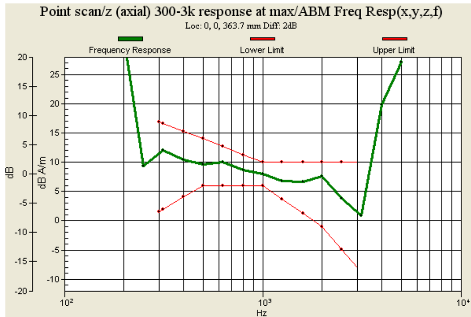
Fig. 9.5: Frequency Response of CDMA2000 PCS Ch600
