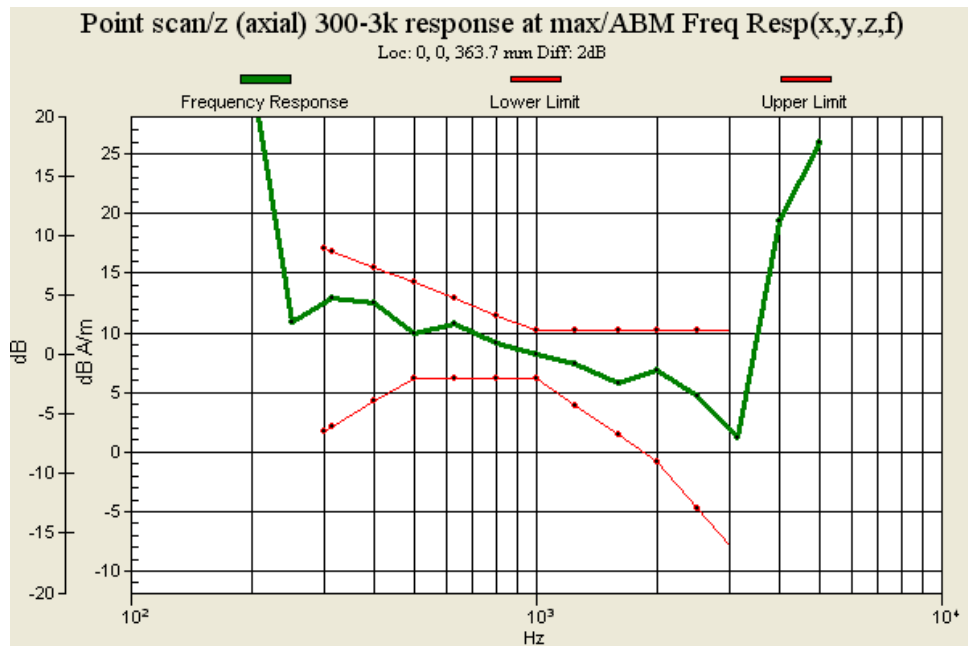
Fig. 9.3: Frequency Response of CDMA2000 Cellular Ch777
