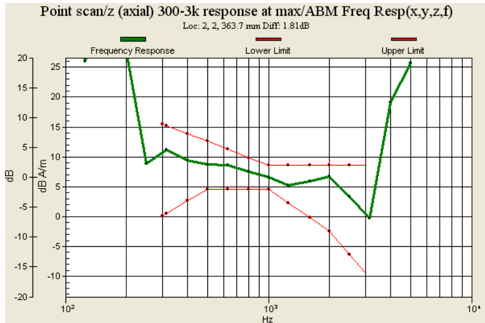
Fig. 9.1: Frequency Response of CDMA2000 Cellular Ch1013
