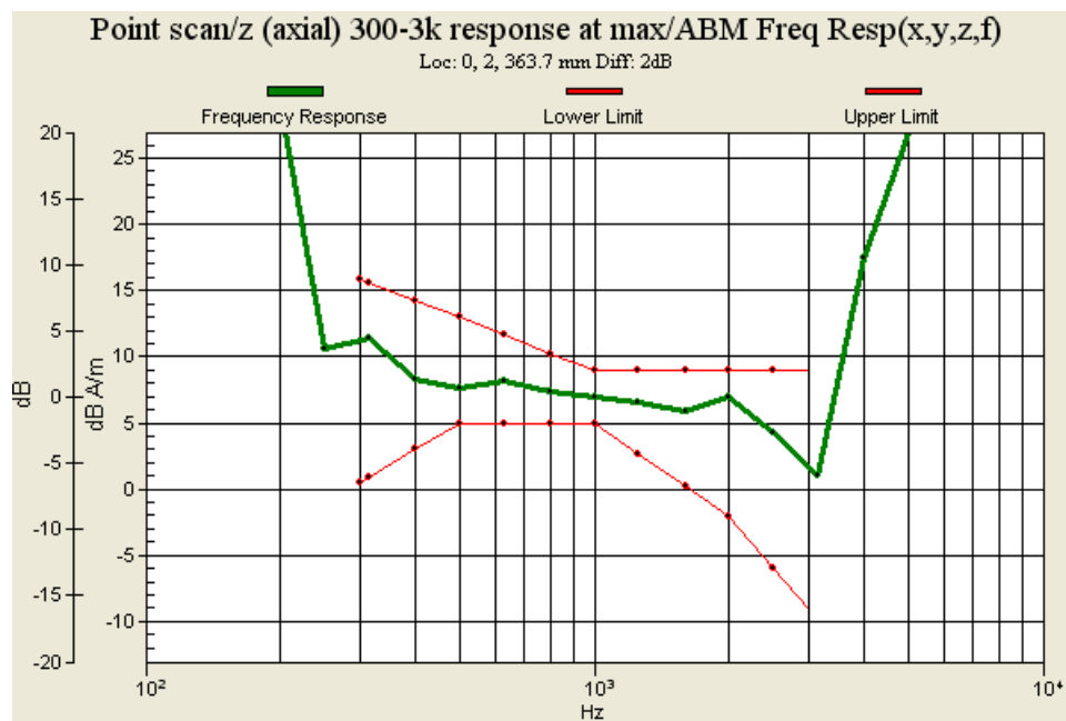
Fig. 9.6: Frequency Response of CDMA2000 PCS Ch1175
