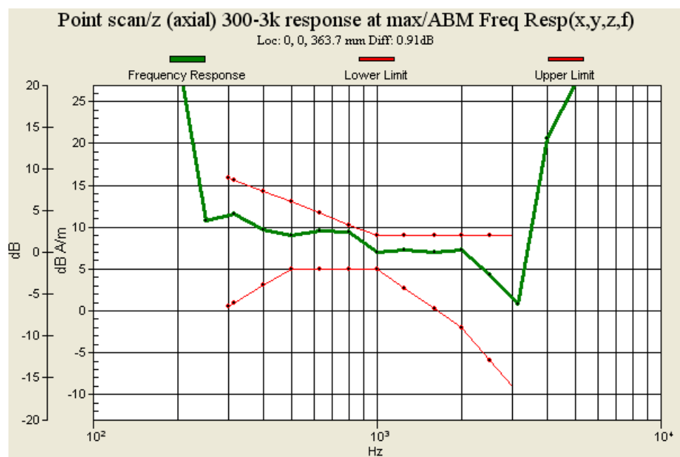
Fig. 9.4: Frequency Response of CDMA2000 PCS Ch25
