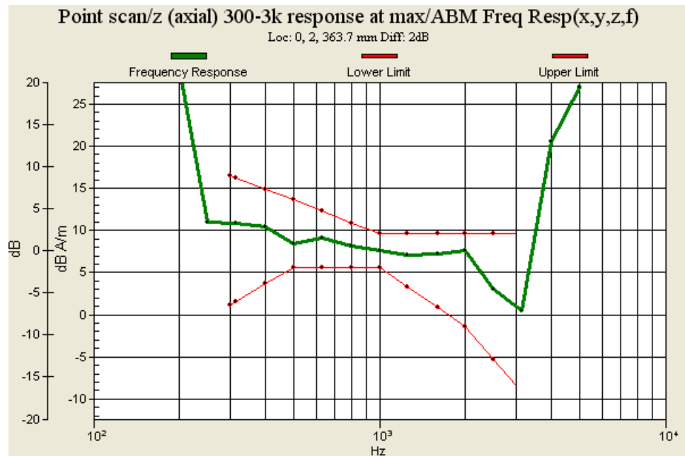
Fig. 9.2: Frequency Response of CDMA2000 Cellular Ch384
