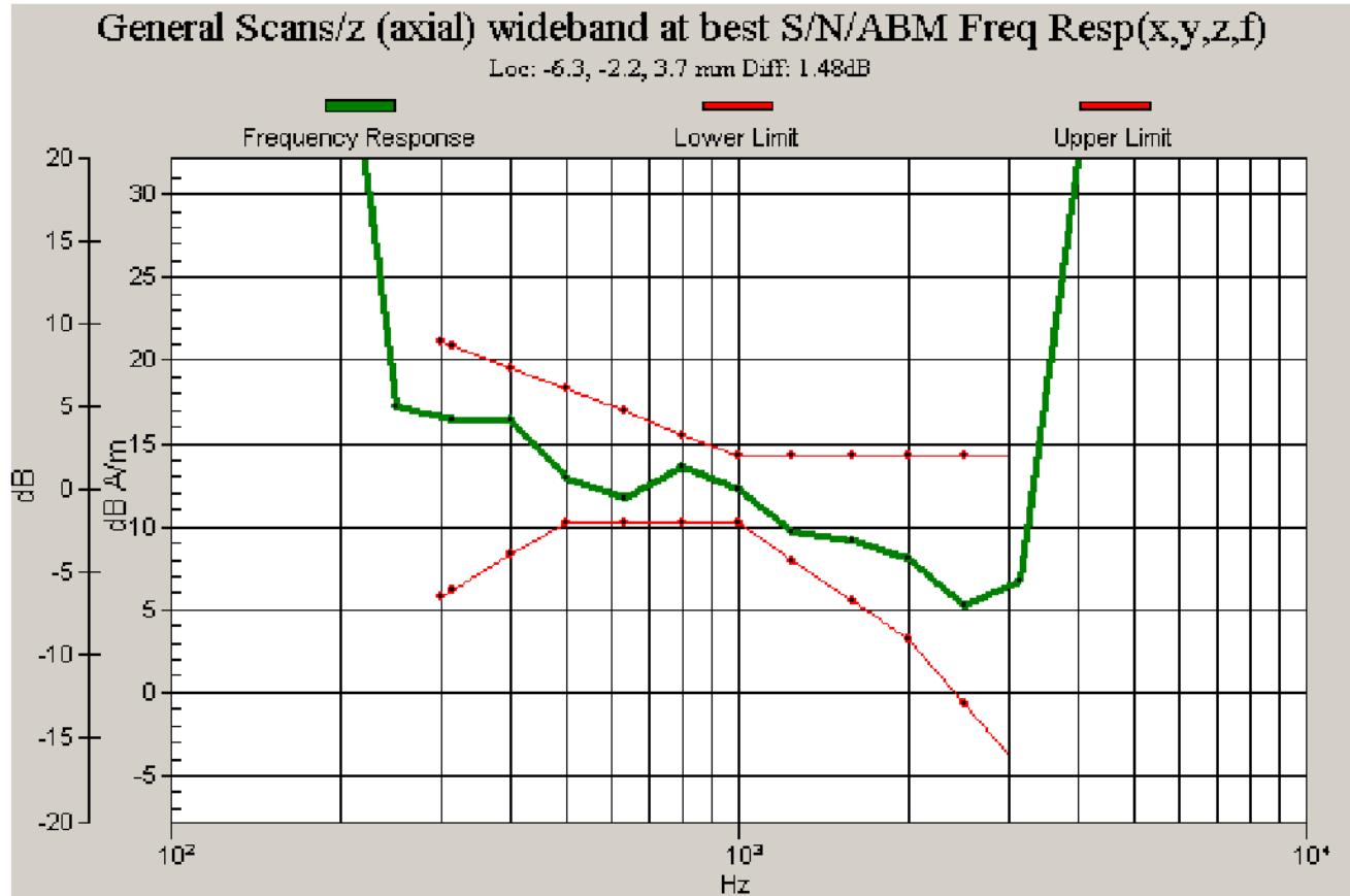
Frequency Response Middle Channel
