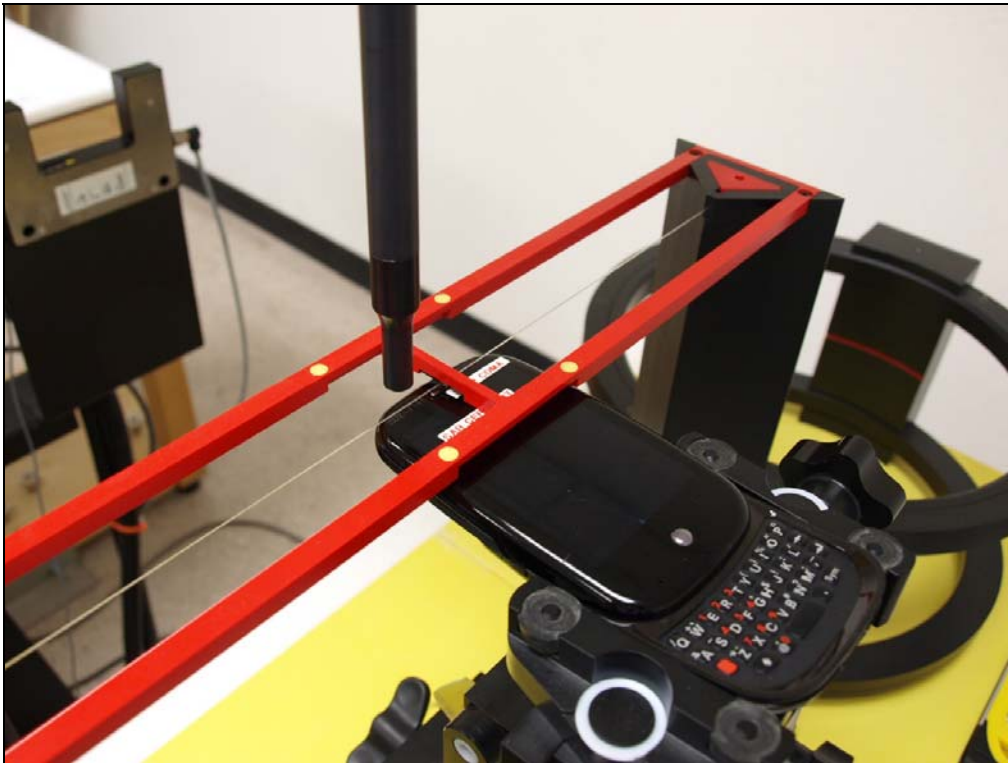
SETUP PHOTO WITH SLIDE OPEN
