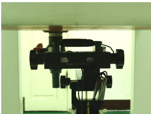
Bottom of the DUT with Phantom 1.5 cm Gap for DUT Slide Off
