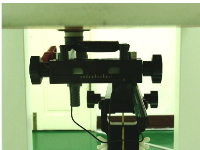
Face of the DUT with Phantom 1.5 cm Gap for DUT Slide Off
