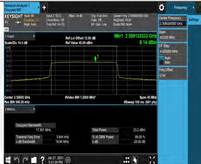
Band41-20MHz-16QAM-39750-100RB#0-17.901
