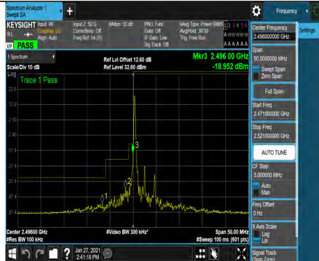
Band41-5MHz-QPSK-39675-1RB#24
